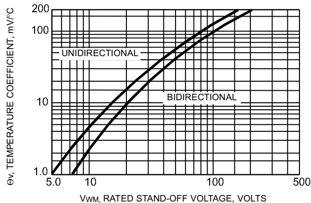
FIG. 12 - BREAKDOWN VOLTAGE TEMPERATURE COEFFICIENT CURVE
