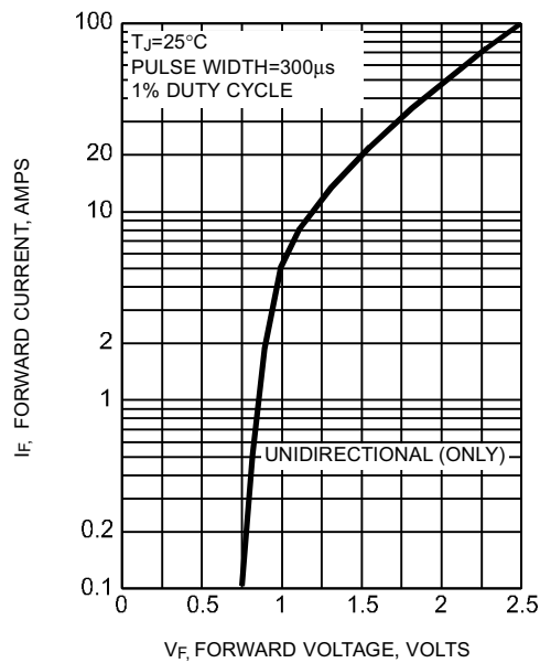
FIG. 11 - TYPICAL INSTANTANEOUS FORWARD VOLTAGE CHARACTERISTICS CURVE
