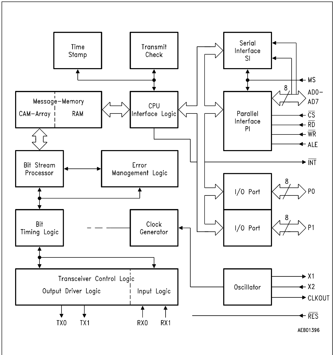
Figure 3 Block Diagram
