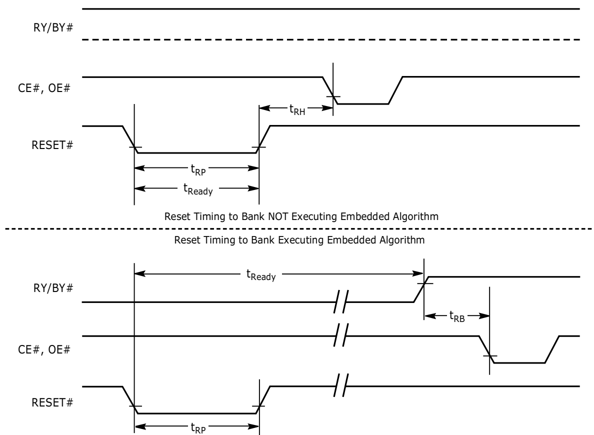
Figure I9. RESET# Timings
