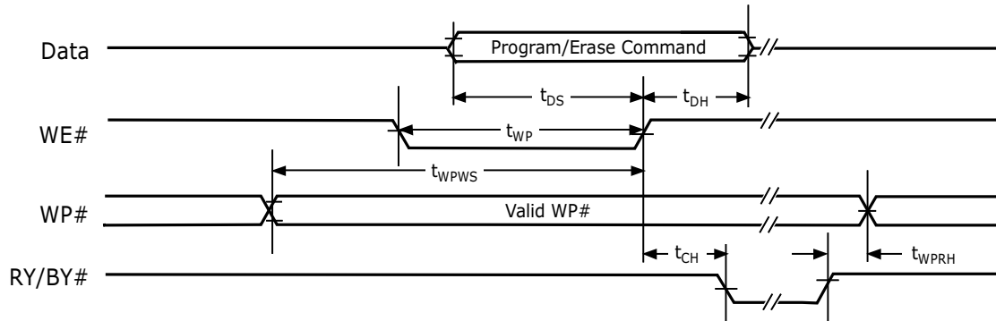
Figure 20. WP# Timing
