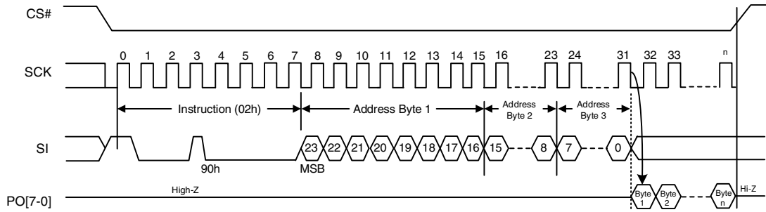
Figure 11.15 Parallel Page Program (PP) Instruction Sequence
