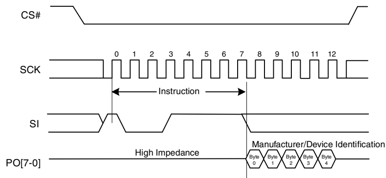
Figure 11.5 Parallel Read_ID Command Sequence and Data Out Sequence
