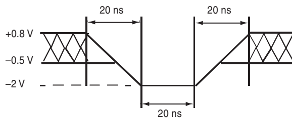
Figure 15.1 Maximum Negative Overshoot Waveform
