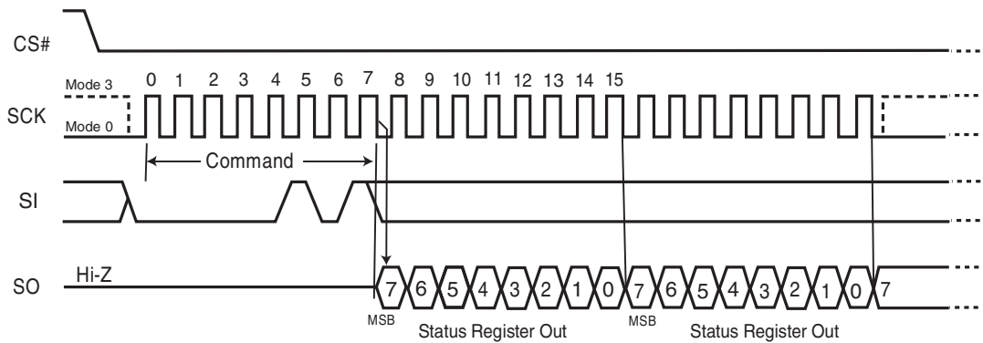
Figure 11.10 Read Status Register (RDSR) Command Sequence
