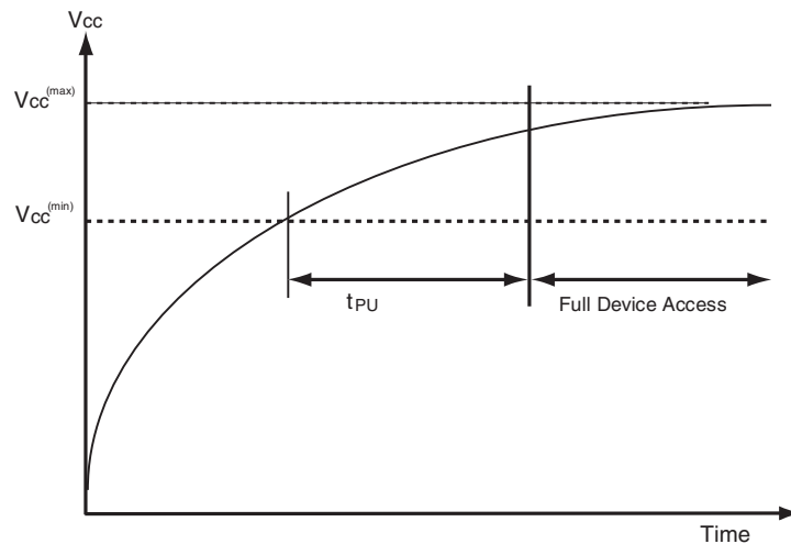
Figure 13.1 Power-Up Timing Diagram
