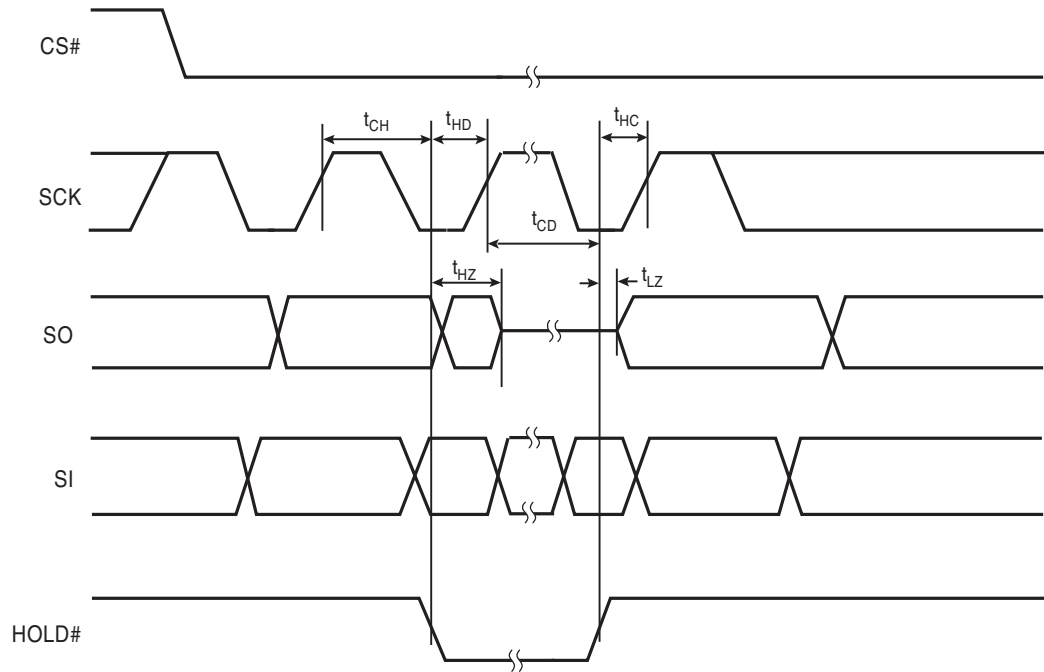
Figure 19.3 HOLD# Timing
