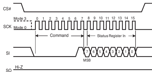
Figure 11.12 Write Status Register (WRSR) Command Sequence
