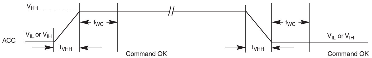
Figure 12.1 ACC Program Acceleration Timing Requirements
