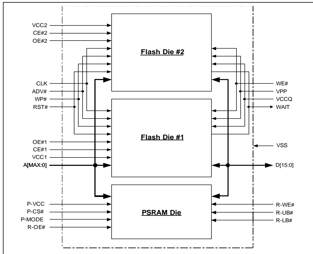
Figure 2. Block Diagram
