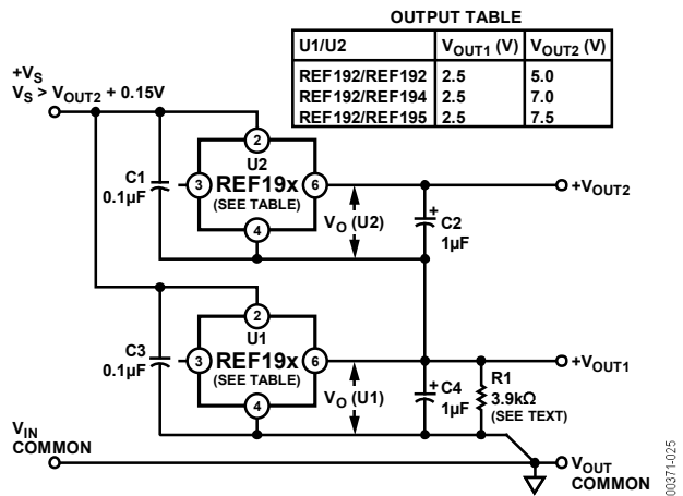
Figure 25. Stacking Voltage References with the REF19x
