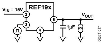
Figure 17. SLEEP Response Time Measurement Circuit
