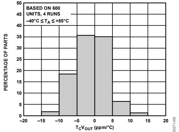
Figure 6. T_cV_{OUT} Distribution
