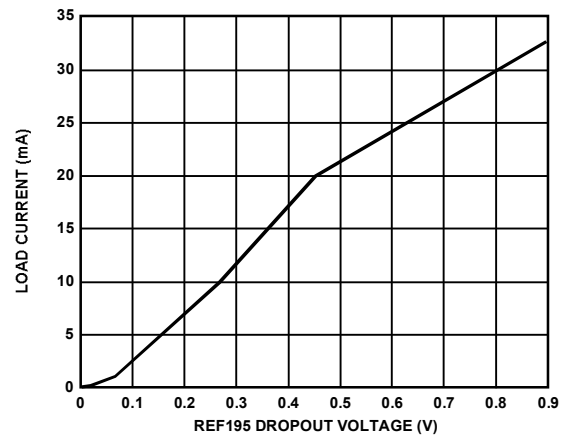
Figure 19. Load Current vs. REF195 Dropout Voltage
