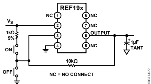
Figure 22. Membrane Switch Controlled Power Supply
