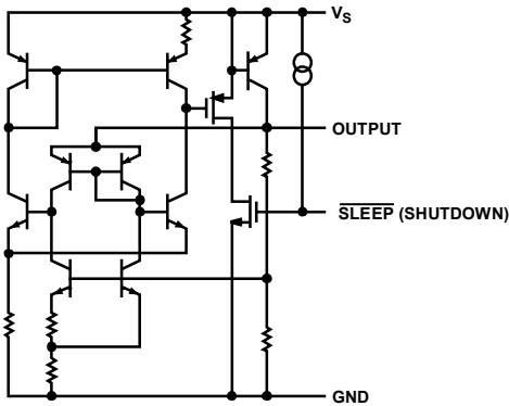
Figure 20. Simplified Schematic
