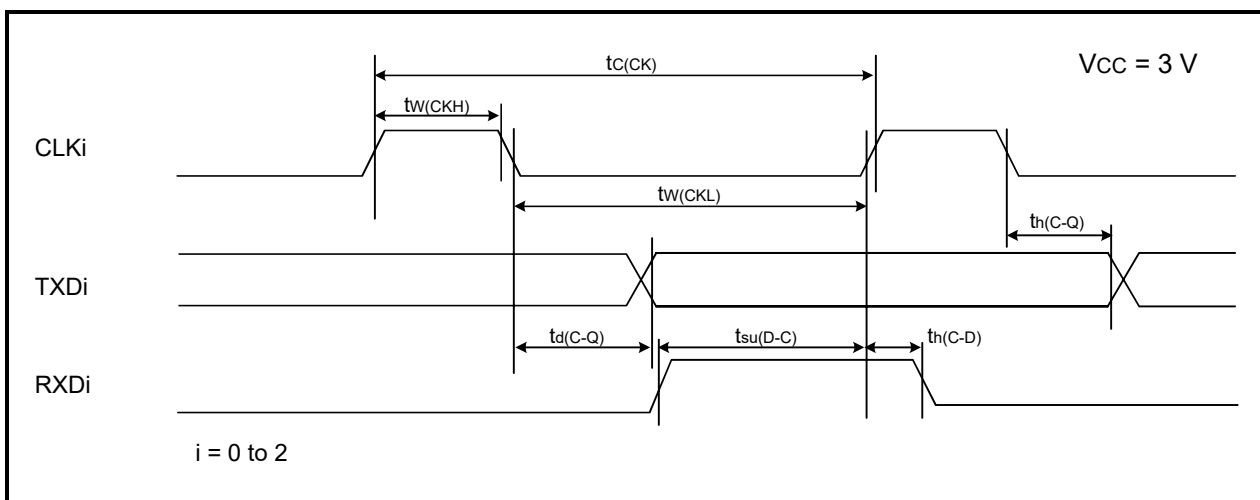
Figure 5.14 Serial Interface Timing Diagram when V_{cc} = 3\text{ V}
