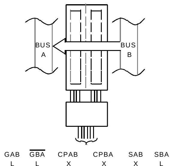
REAL-TIME TRANSFER BUS B TO A
