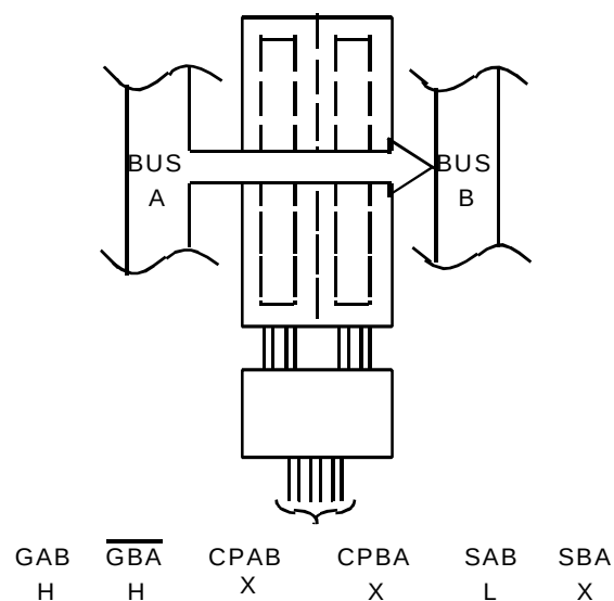
REAL-TIME TRANSFER BUS A TO B
