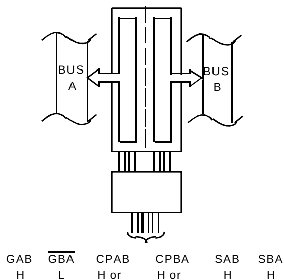
TRANSFER STORES DATA TO A AND/OR B
