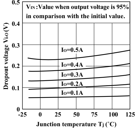
Fig.10 Dropout Voltage vs. Junction Temperature (PQ3TZ50/PQ3TZ53)
