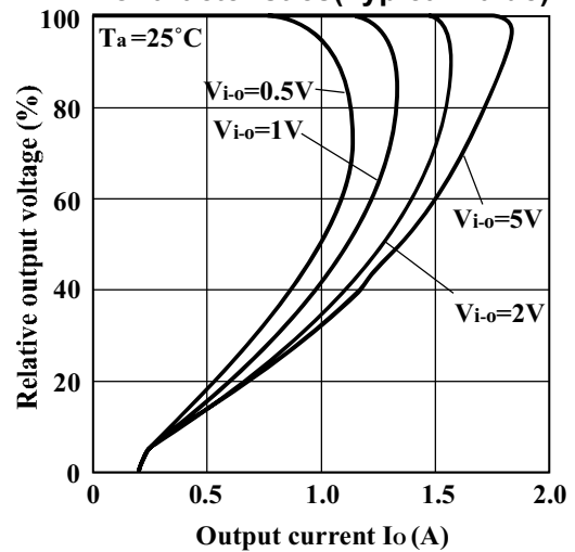
Fig.4 Overcurrent Protection Characteristics(Typical Value)
