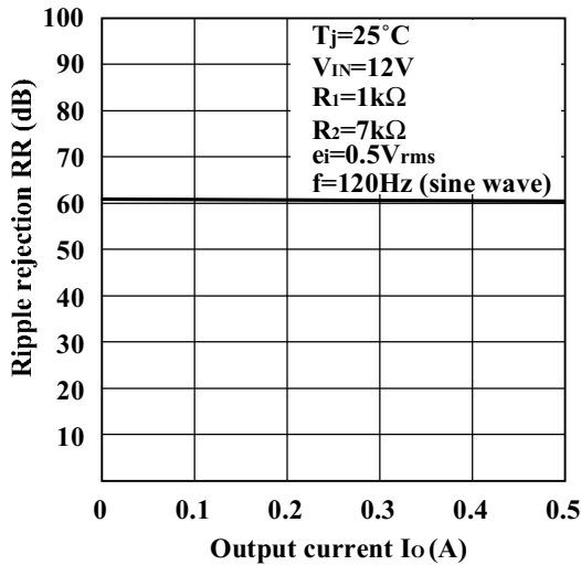
Fig.13 Ripple Rejection vs. Output Current (PQ20VZ51)
