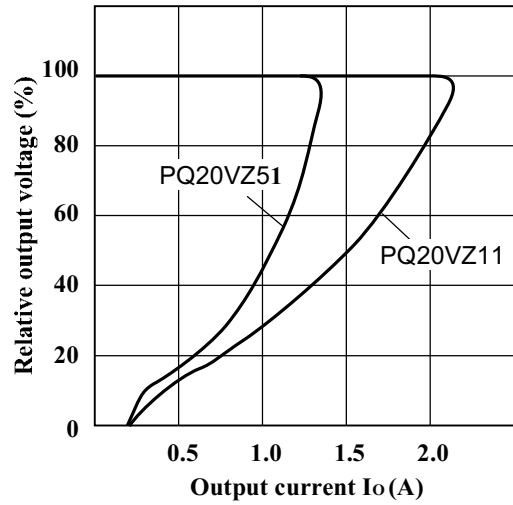
Fig.4 Overcurrent Protection Characteristics (Typical Value)
