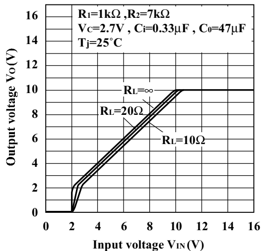
Fig.8 Output Voltage vs. Input Voltage (PQ20VZ11)
