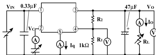
Fig.1 Test Circuit
