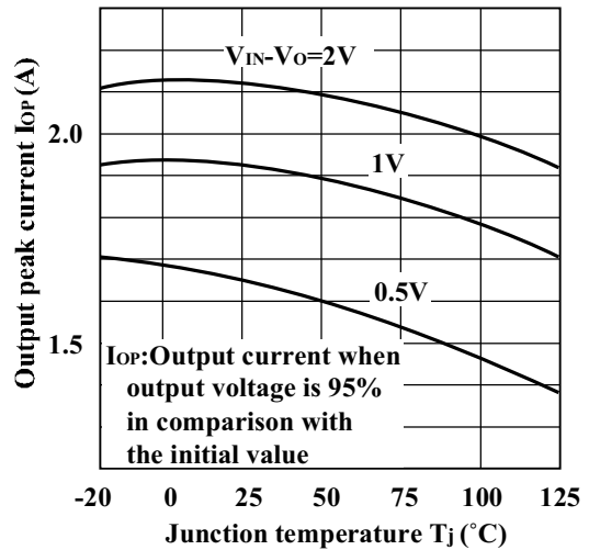
Fig.18 Output Peak Current vs. Junction Temperature (PQ20VZ11)
