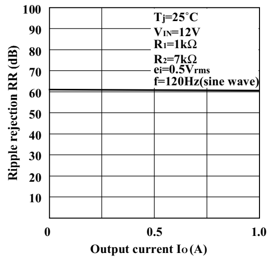
Fig.14 Ripple Rejection vs. Output Current (PQ20VZ11)
