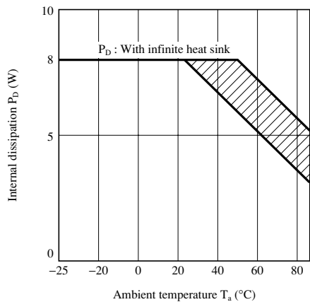
Fig.4 Internal Dissipation vs. Ambient Temperature
