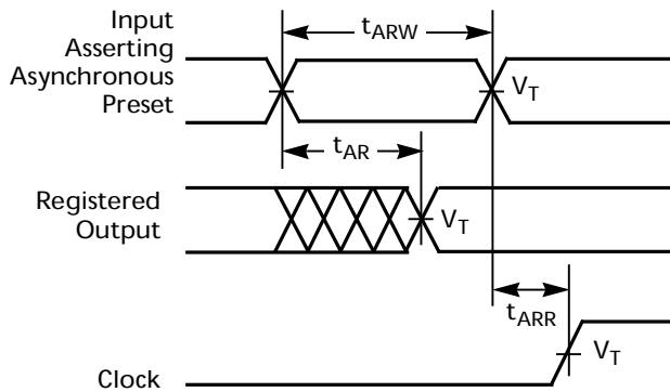
e. Asynchronous reset
