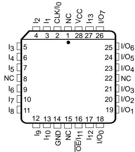
PLCC/LCC
