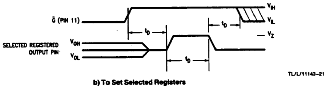
FIGURE 2. Register Preload Waveforms
