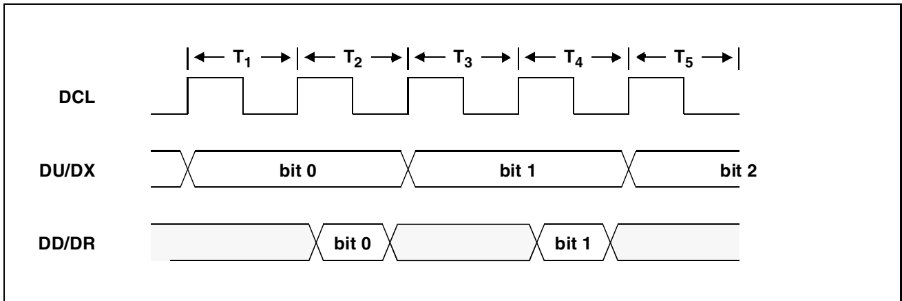
Figure 41 IOM ® -2 Interface - Double Clock Mode
