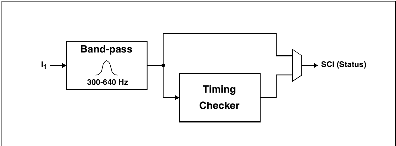
Figure 16 CPT Detector - Block Diagram
