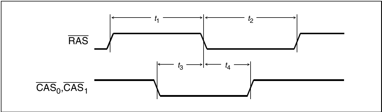
Figure 75 Memory Interface - DRAM Refresh Cycle
