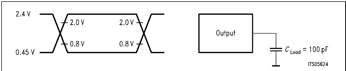
Figure 66 Input/Output Waveforms for AC-Tests
