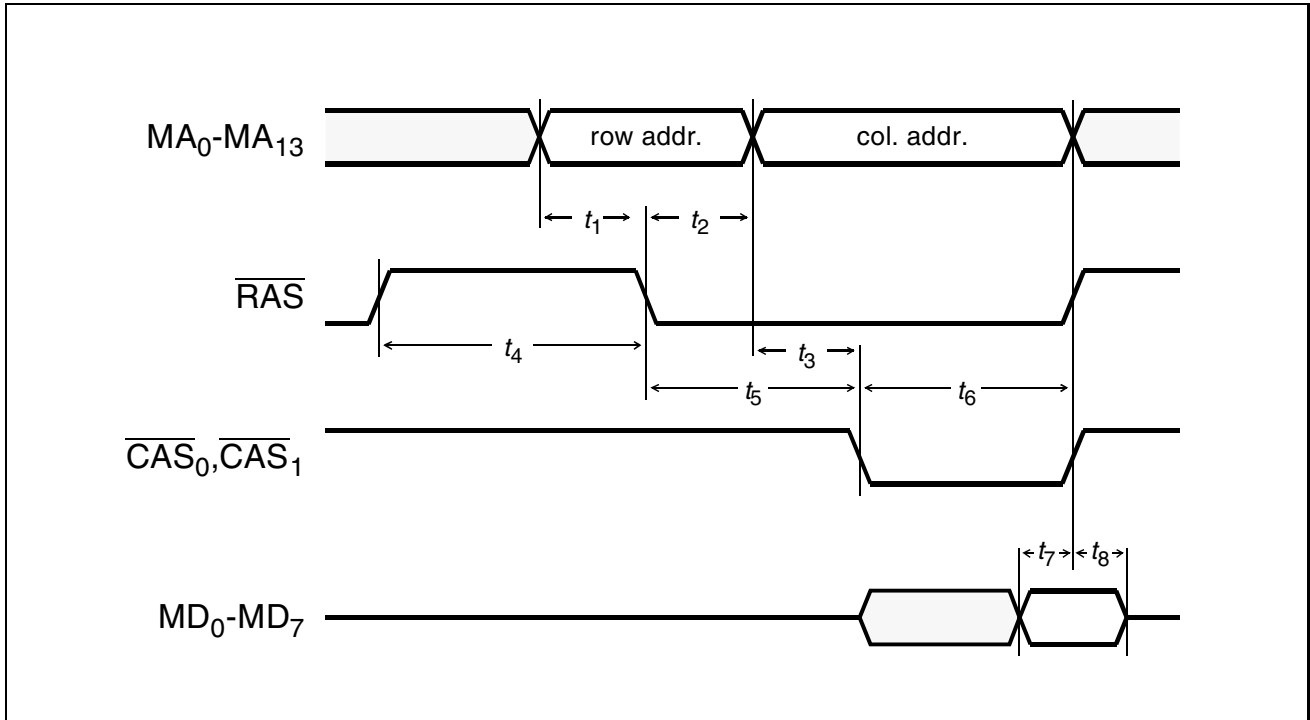
Figure 73 Memory Interface - DRAM Read Access
