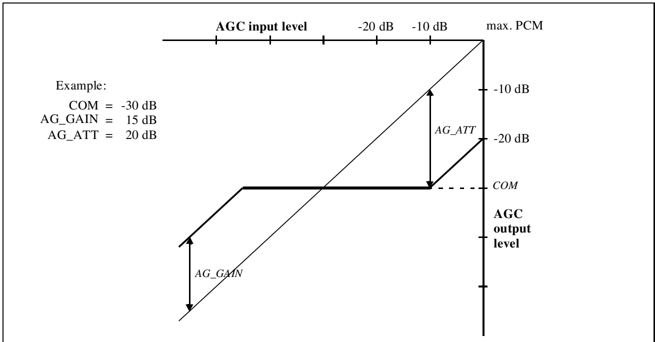
Figure 28 Echo Suppression Unit - Automatic Gain Control
