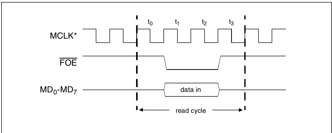
Figure 61 Parallel Flash Memory Interface - Data Read
