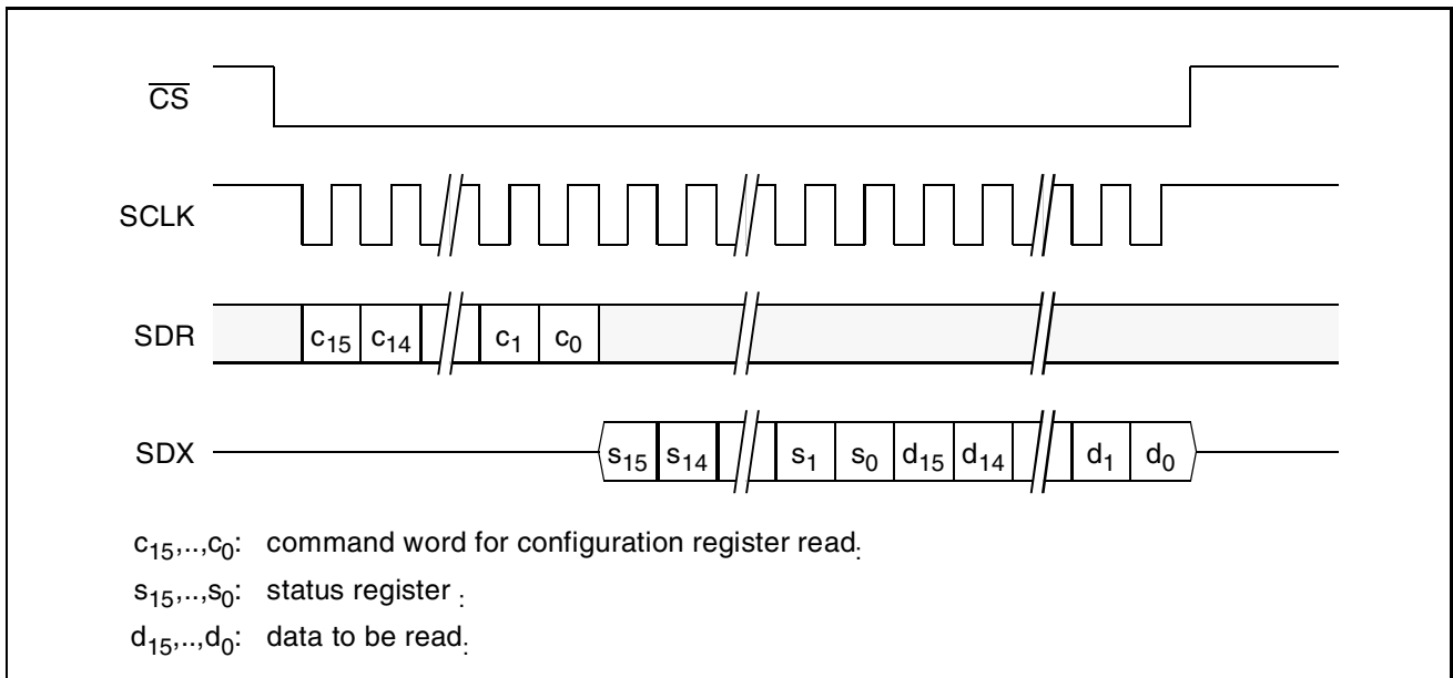
Figure 49 Configuration Register Read Access
