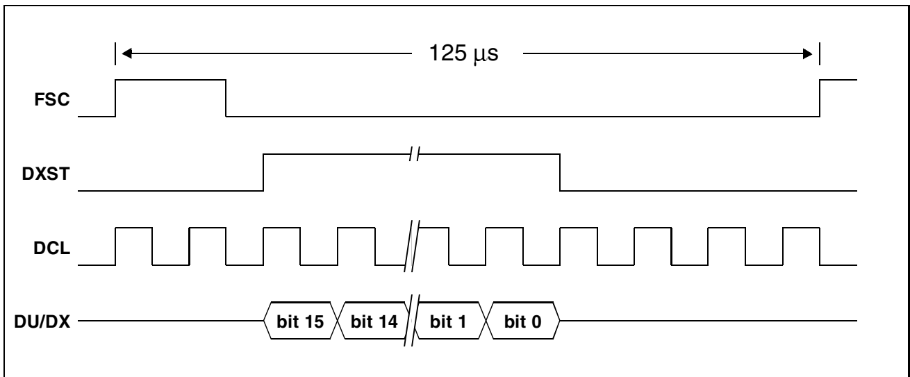
Figure 43 SSDI Interface - Transmitter Timing
