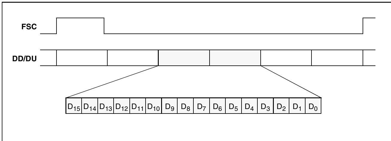
Figure 42 IOM ® -2 Interface - Channel Structure
