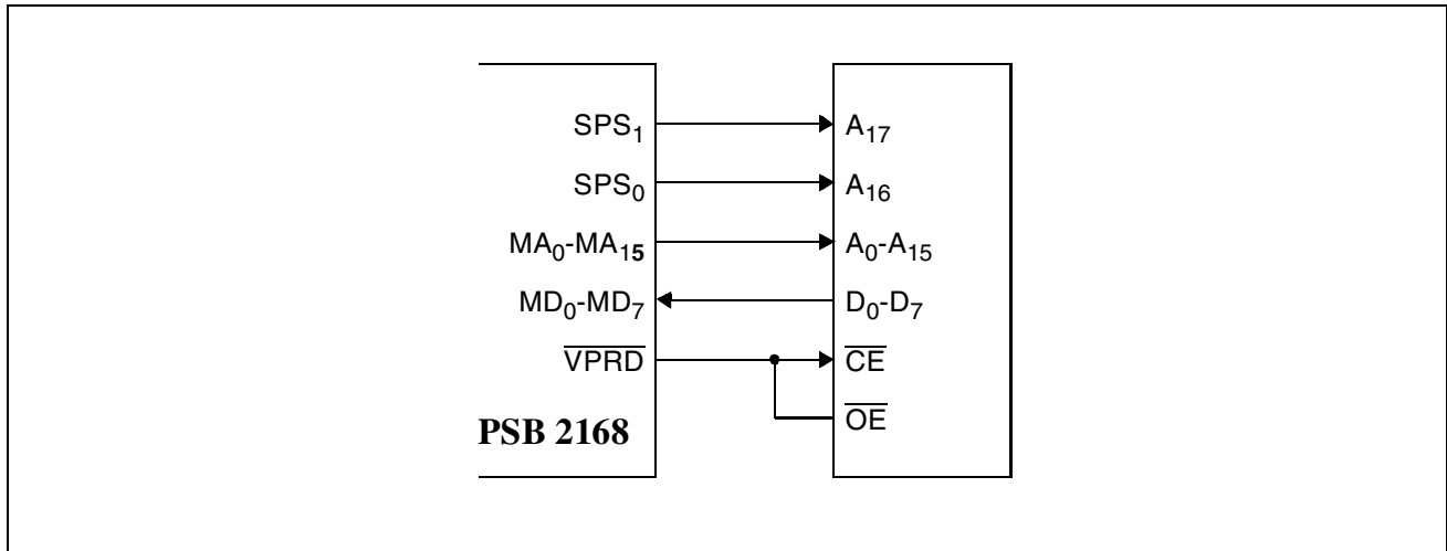
Figure 55 EPROM Interface - Connection Diagram
