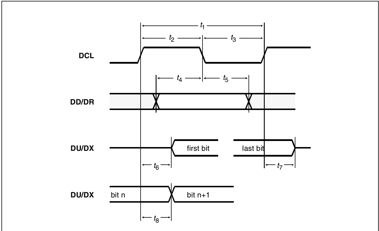
Figure 68 SSDI/IOM ® -2 Interface - Bit Synchronization Timing
