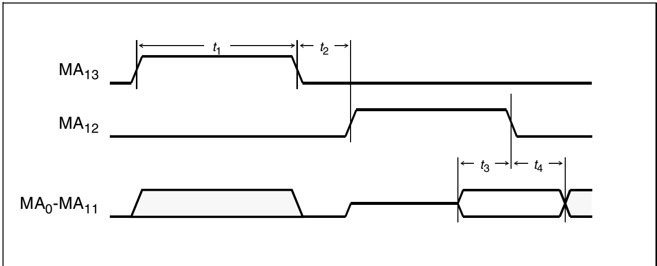
Figure 81 Auxiliary Parallel Port - Multiplex Mode
