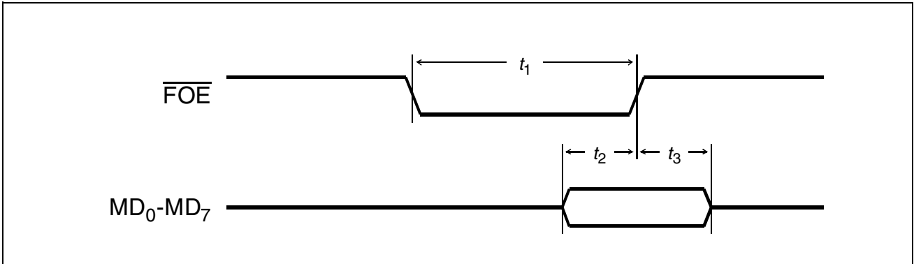
Figure 80 Memory Interface - Samsung Data Read
