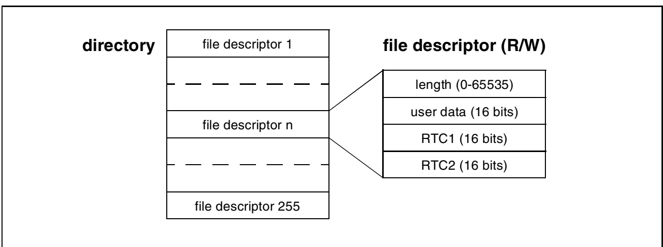
Figure 32 Memory Management - Structure of Message Directory
