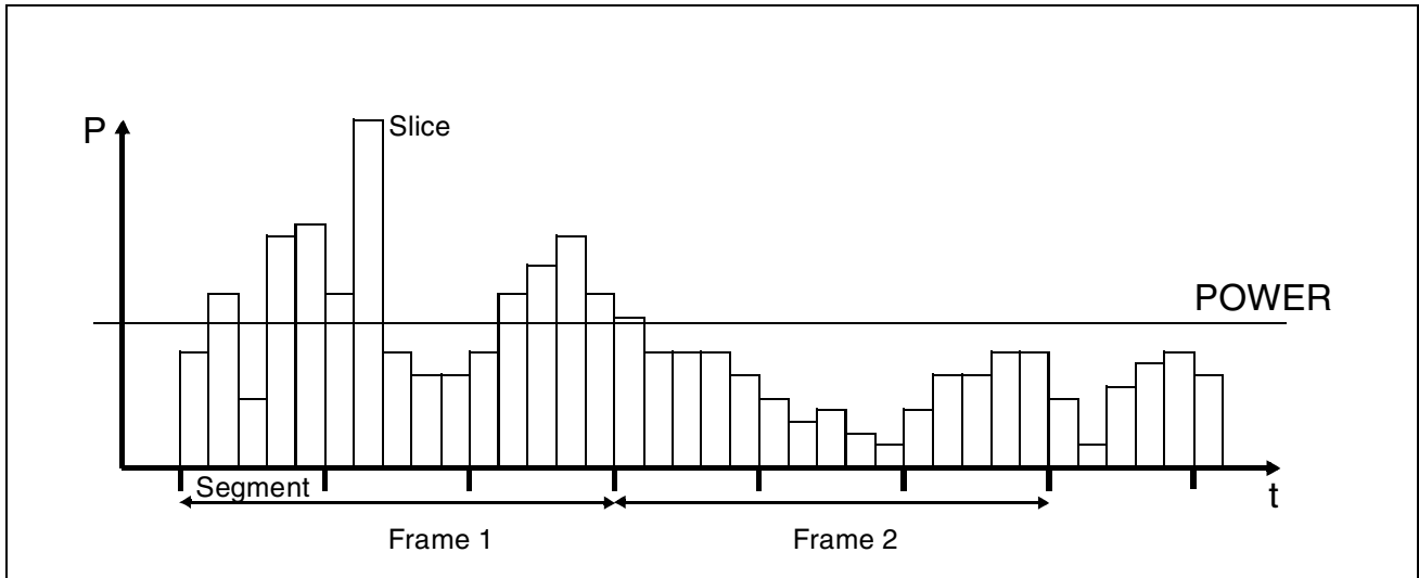
Figure 23 VOX Detector
