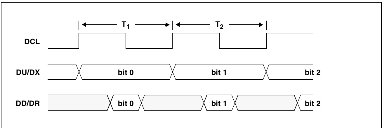
Figure 40 IOM ® -2 Interface - Single Clock Mode
