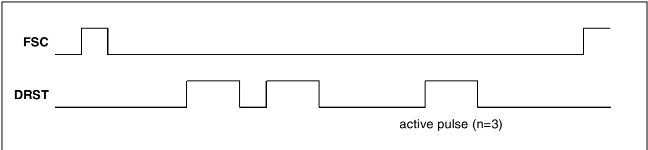
Figure 44 SSDI Interface - Active Pulse Selection
