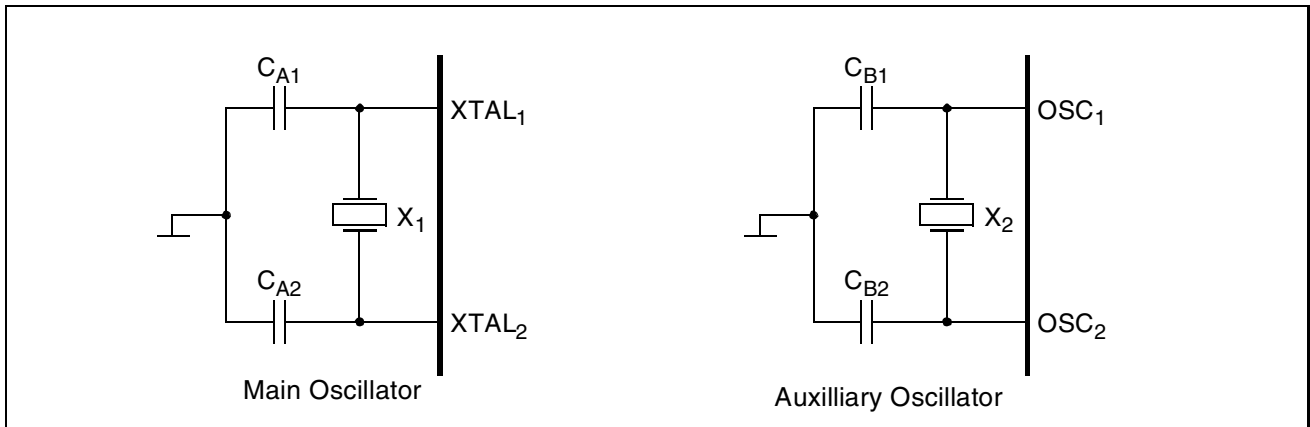
Figure 67 Oscillator Circuits
