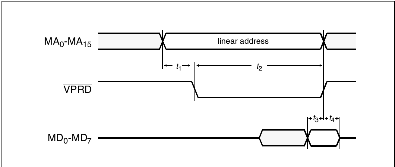
Figure 76 Memory Interface - EPROM Read
