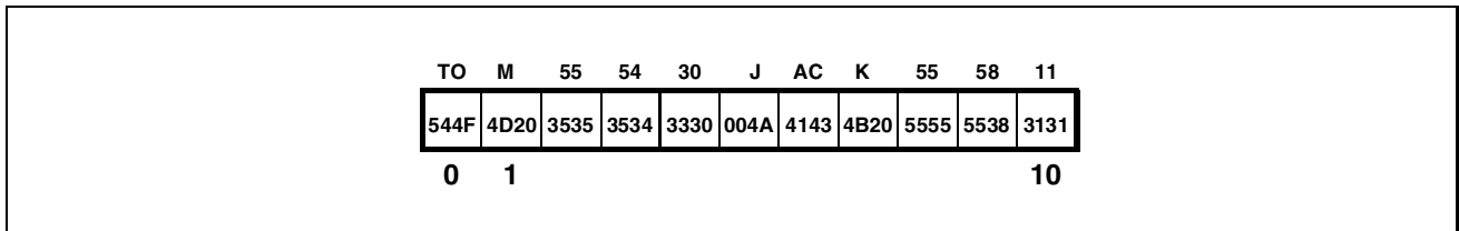
Figure 35 Binary File Organization - Example
