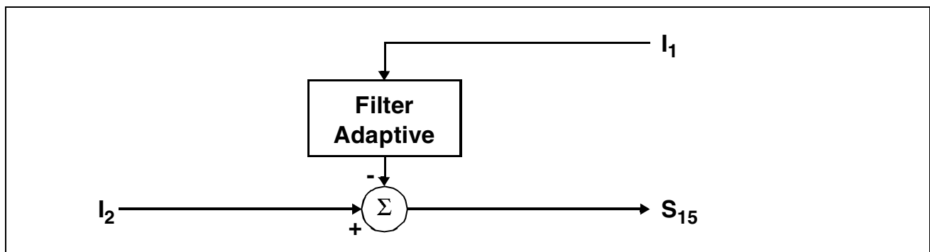
Figure 10 Line Echo Cancellation Unit - Block Diagram
