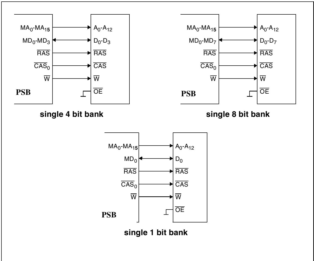
Figure 51 ARAM/DRAM Interface - Connection Diagram
