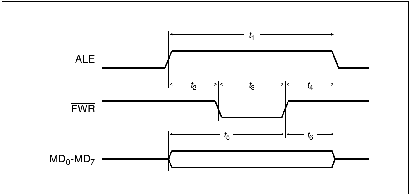
Figure 78 Memory Interface - Samsung Address Write
