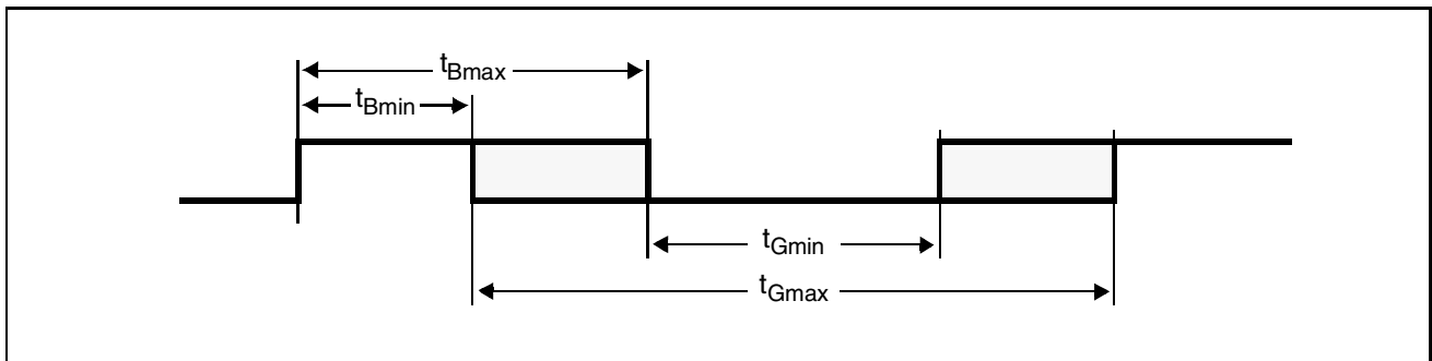
Figure 17 CPT Detector - Cooked Mode
