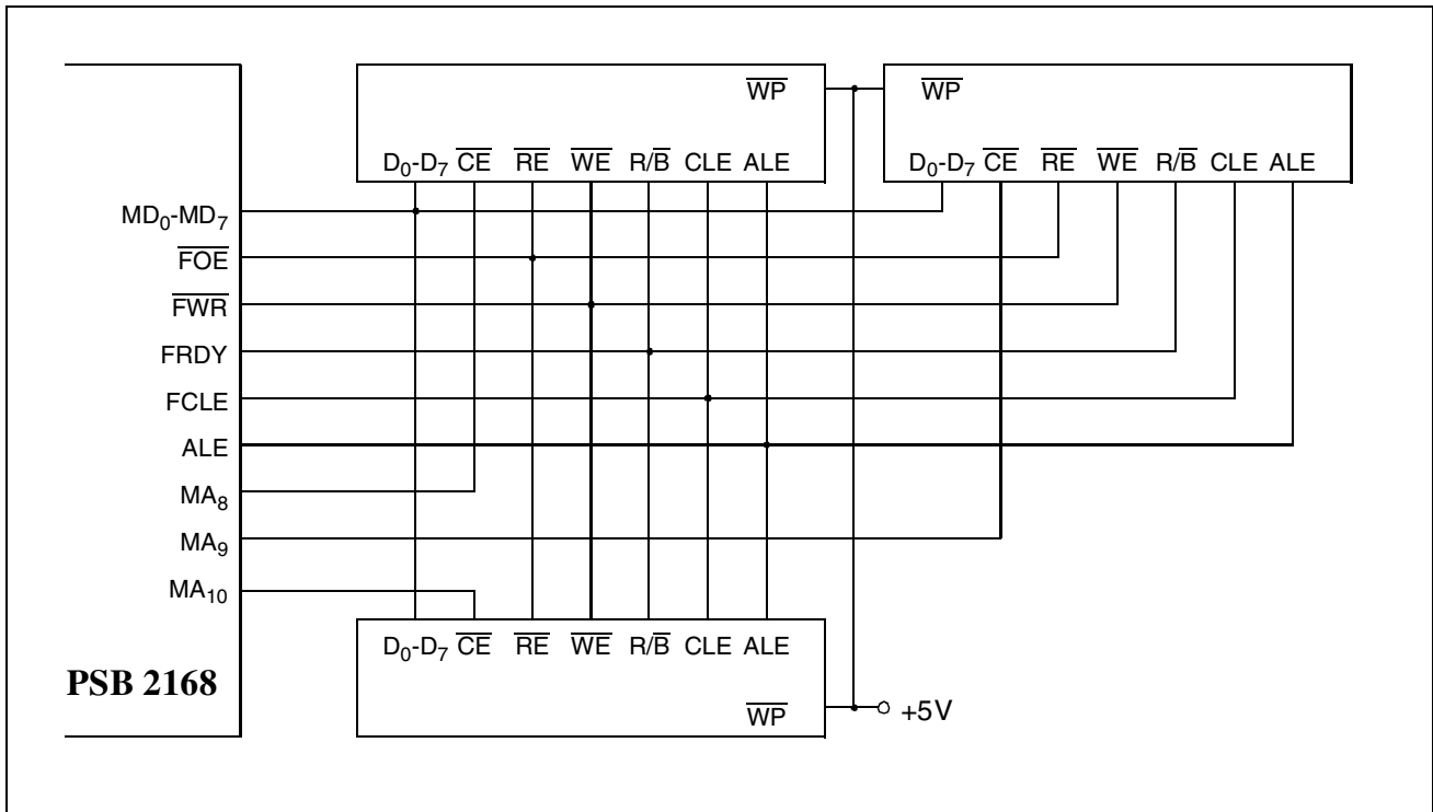
Figure 57 Parallel Flash Memory Interface - Multiple Devices
