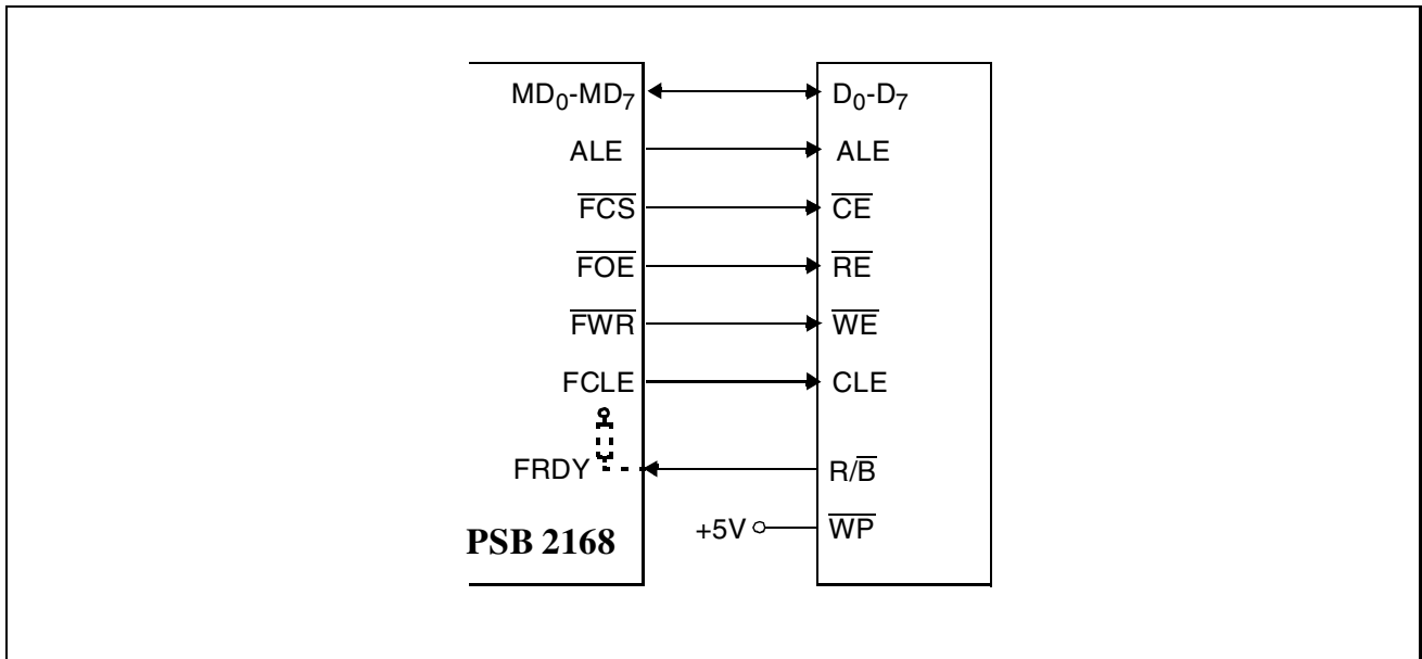
Parallel Flash Memory Interface - Connection Diagram
