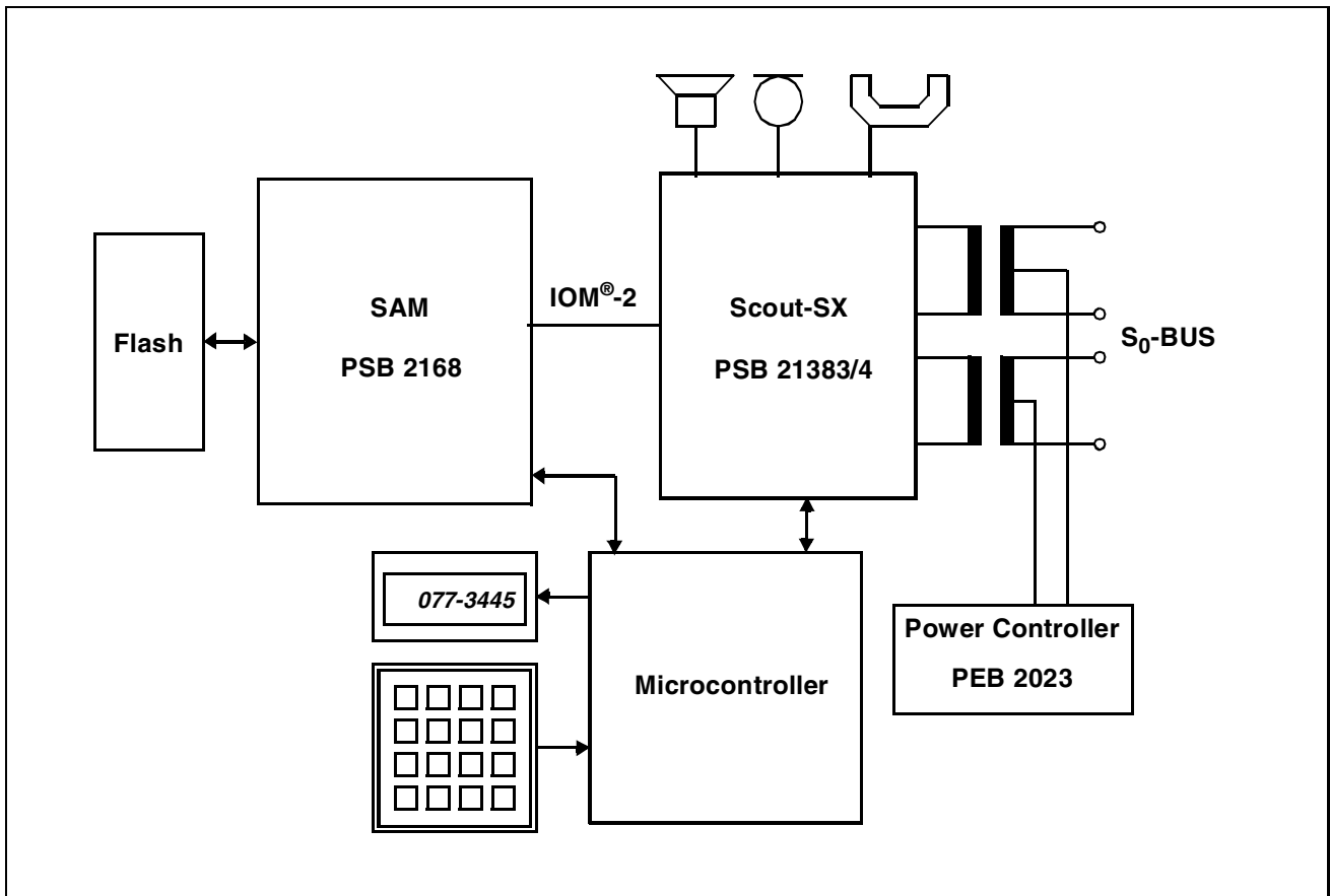
Figure 4 Featurephone with Answering Machine for ISDN Terminal
