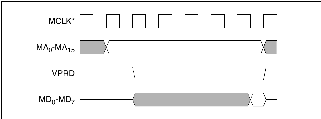
Figure 56 EPROM Interface - Read Cycle Timing
