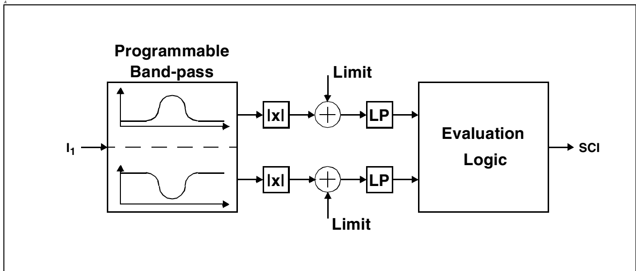
Figure 15 Universal Tone Detector - Block Diagram
