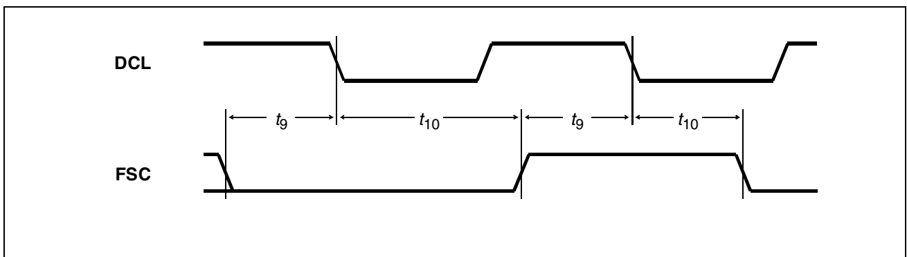
Figure 69 SSDI/IOM ® -2 Interface - Frame Synchronization Timing
