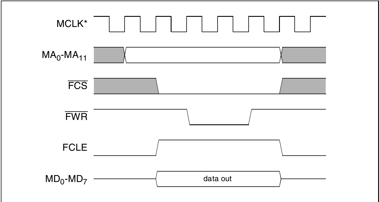
Figure 58 Parallel Flash Memory Interface - Command Write
