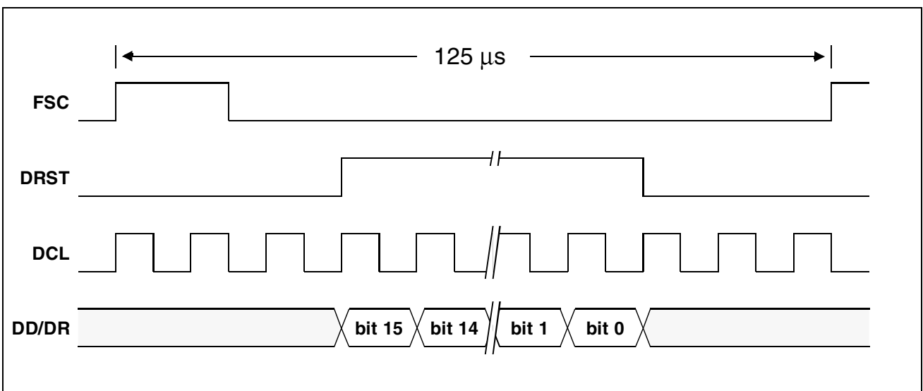
Figure 45 SSDI Interface - Receiver Timing
