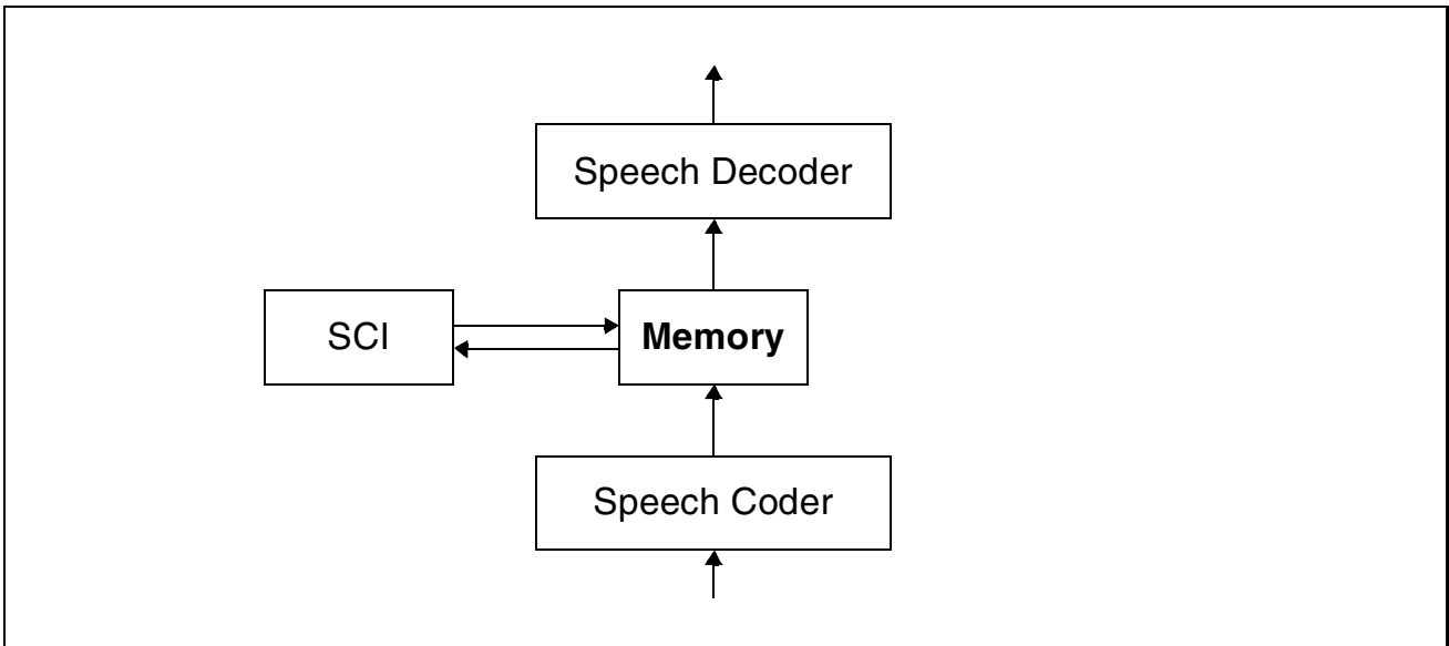
Figure 31 Memory Management - Data Flow
