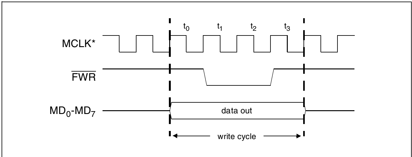
Figure 60 Parallel Flash Memory Interface - Data Write
