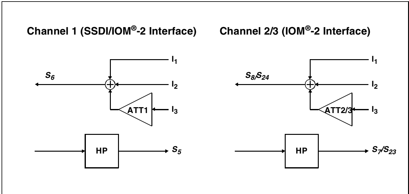
Figure 25 Digital Interface - Block Diagram
