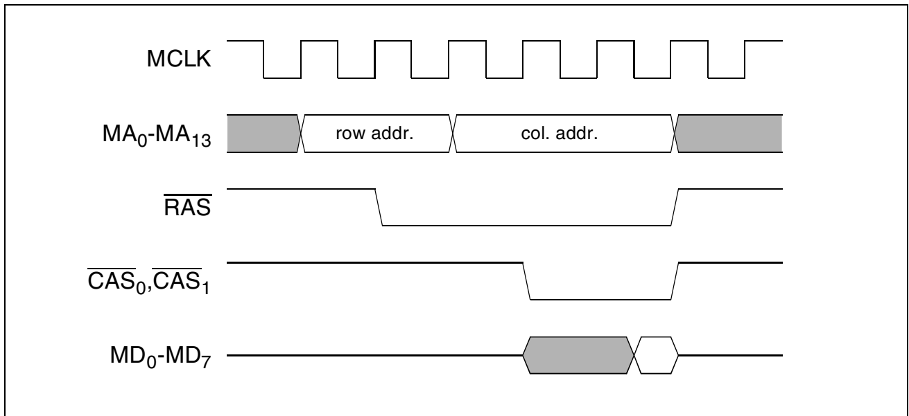
Figure 52 ARAM/DRAM Interface - Read Cycle Timing
