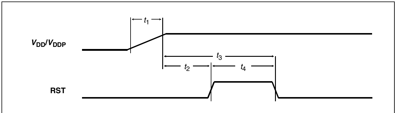
Figure 82 Reset Timing
