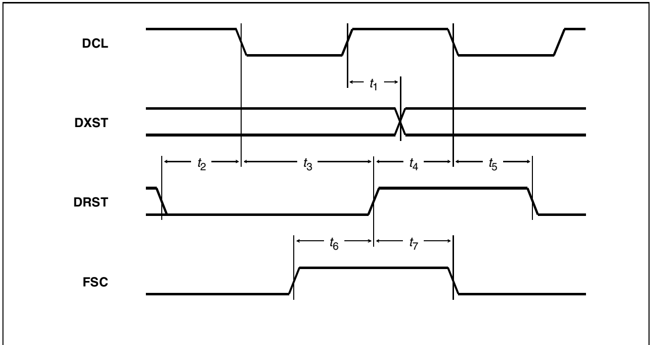
Figure 70 SSDI Interface - Strobe Timing
