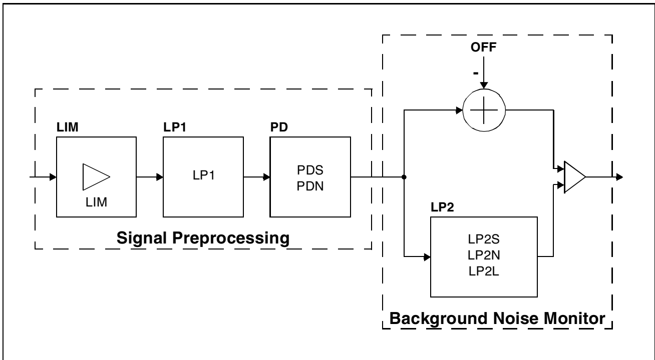
Figure 22 Speech Coder - Speech Detector
