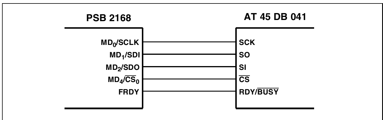
Figure 63 Serial Flash - Connection to Single AT 45 DB 041
