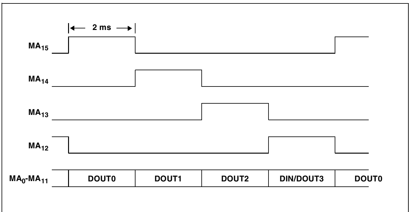
Figure 65 Auxiliary Parallel Port - Multiplex Mode
