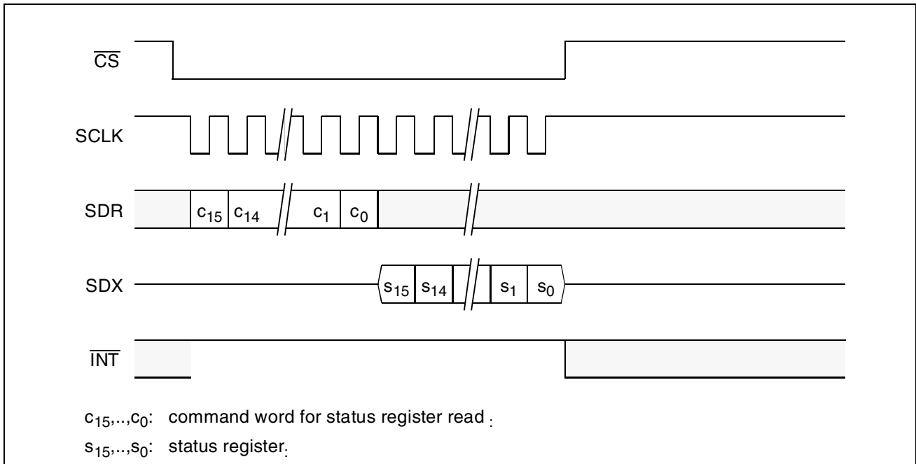
Figure 46 Status Register Read Access
