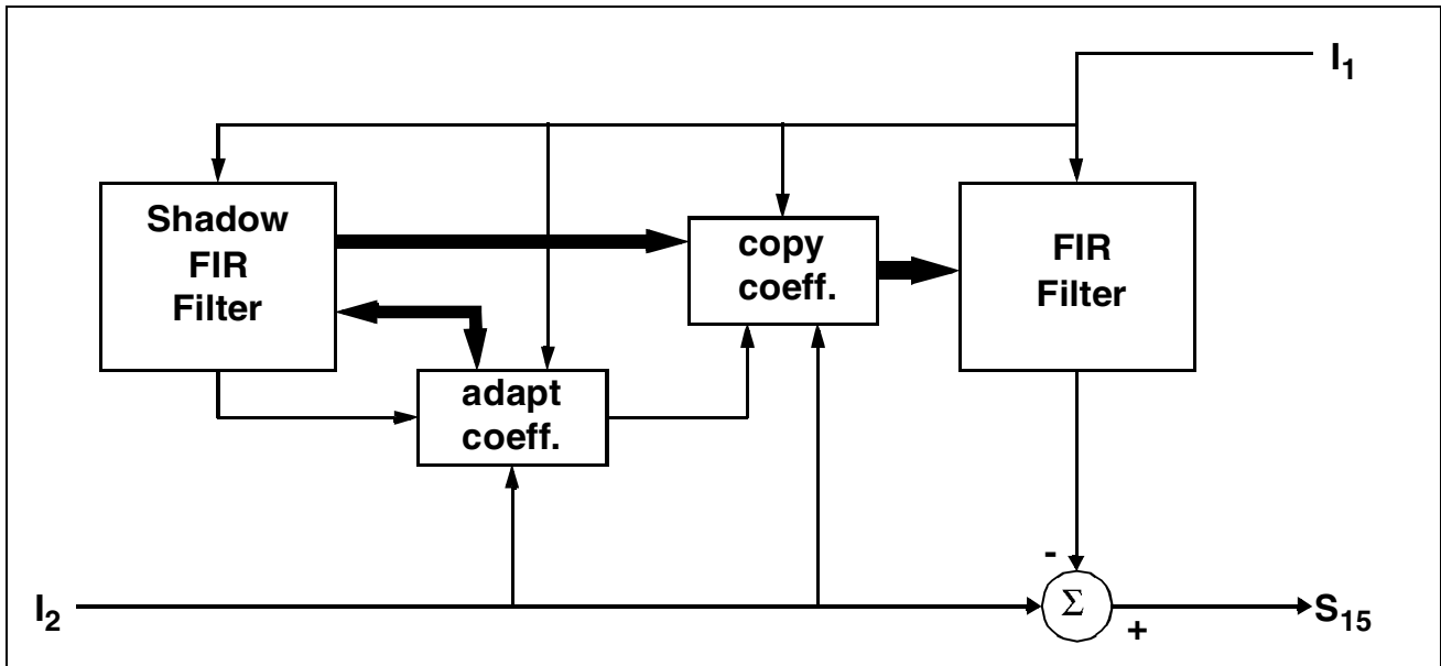
Figure 11 Line Echo Cancellation Unit - Superior Mode with Shadow FIR
