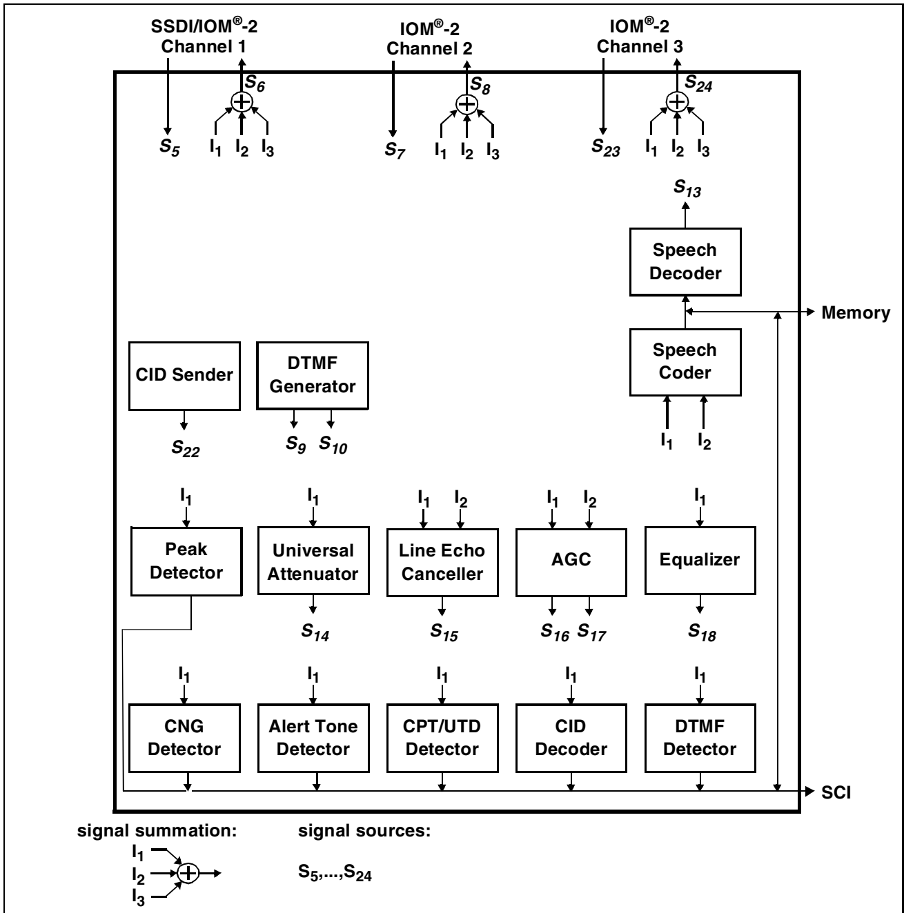
Figure 8 Functional Units - Overview
