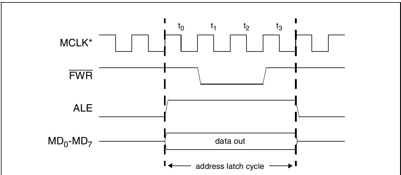
Figure 59 Parallel Flash Memory Interface - Address Write
