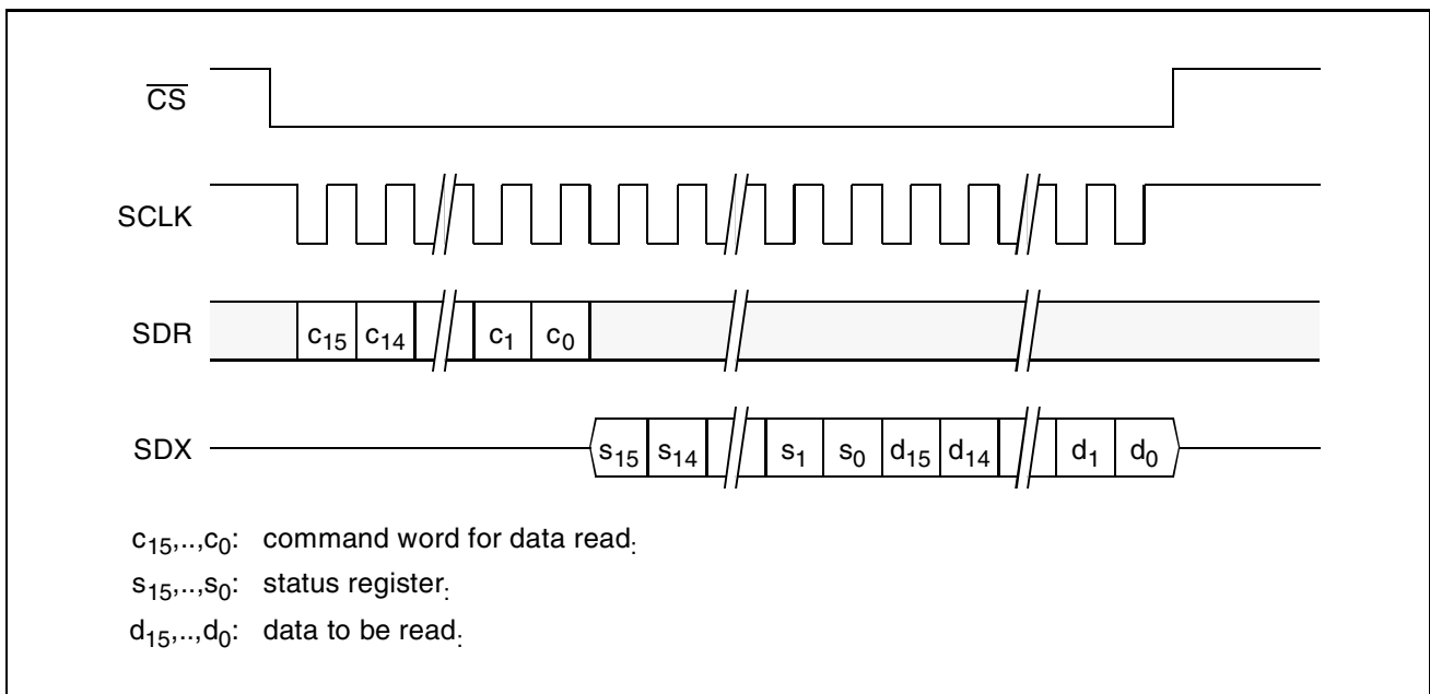
Figure 47 Data Read Access
