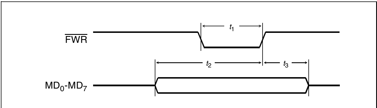
Figure 79 Memory Interface - Samsung Data Write
