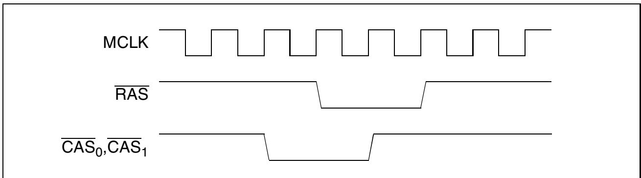
Figure 54 ARAM/DRAM Interface - Refresh Cycle Timing
