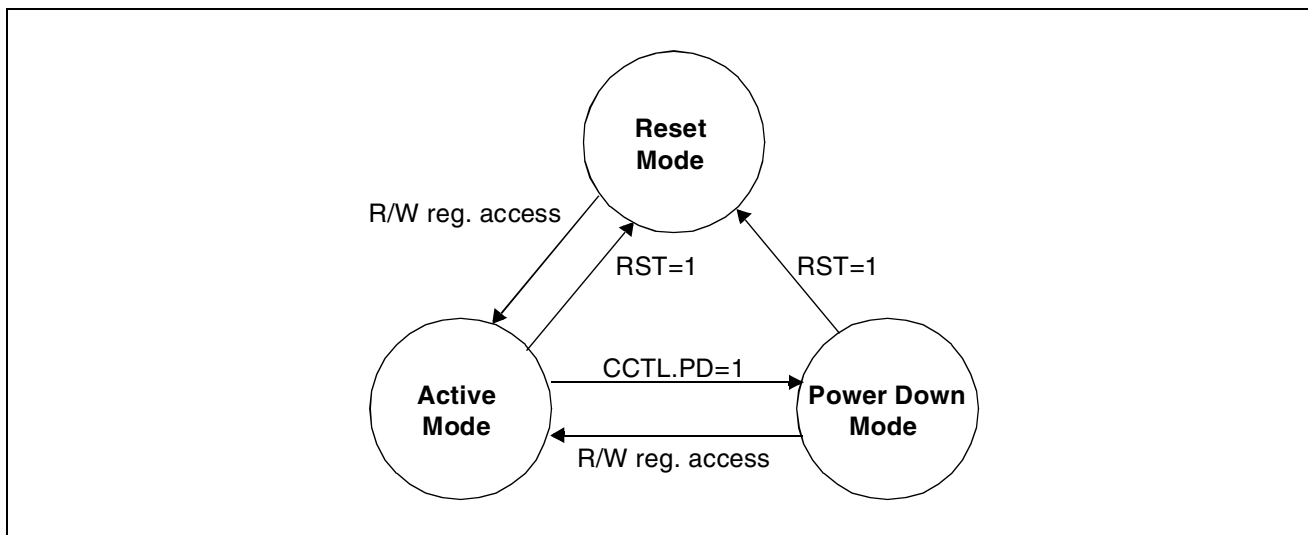
Figure 37 Operation Modes - State Chart
