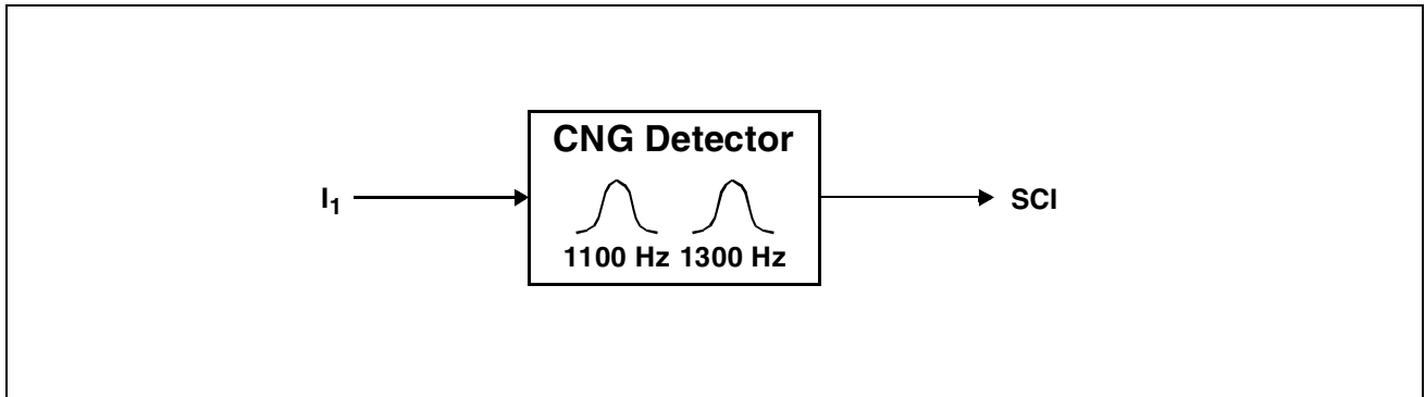
Figure 13 CNG Detector - Block Diagram
