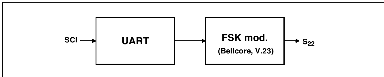
Figure 19 Caller ID Sender - Block Diagram
