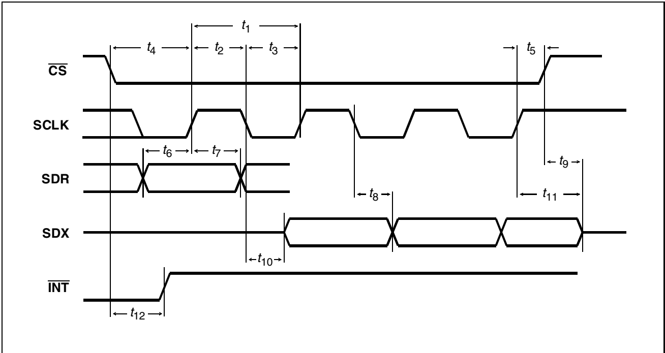
Figure 71 Serial Control Interface
