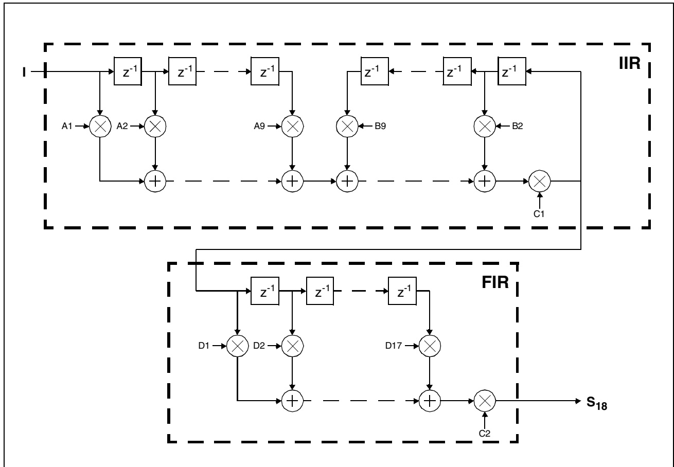
Figure 29 Equalizer - Block Diagram
