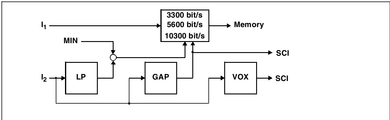
Figure 21 Speech Coder - Block Diagram
