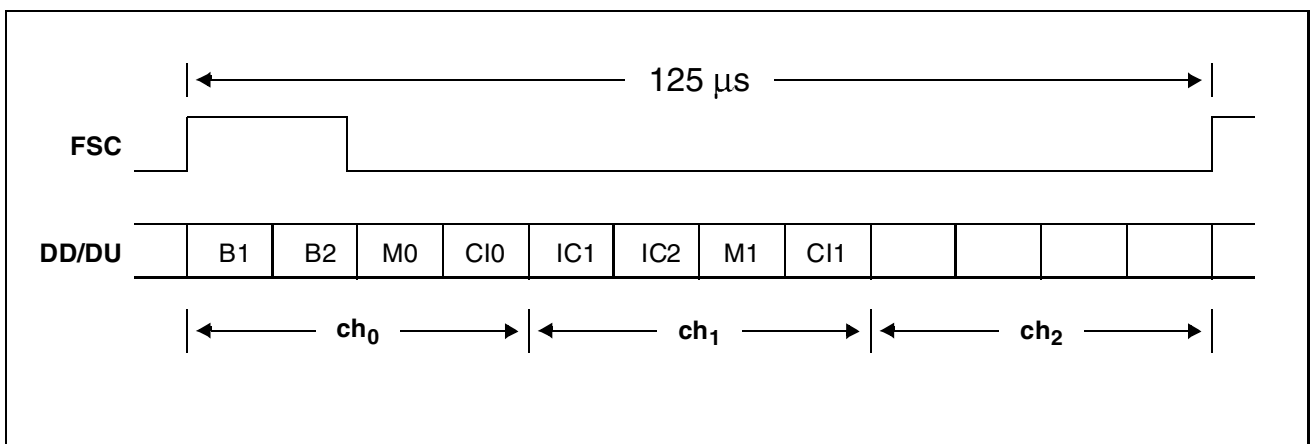
Figure 38 IOM ® -2 Interface - Frame Structure
