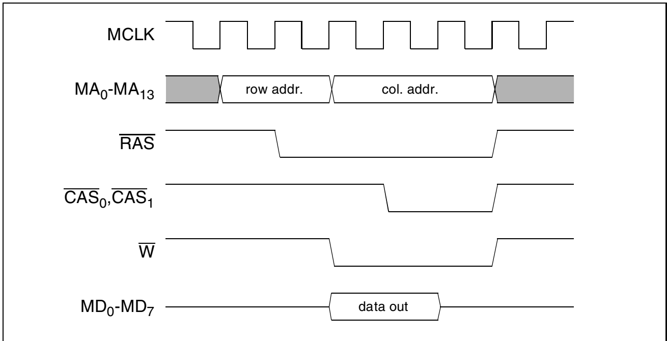
Figure 53 ARAM/DRAM Interface - Write Cycle Timing
