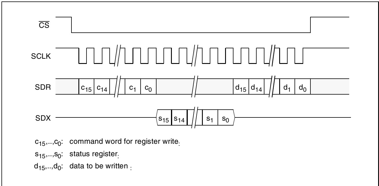
Figure 48 Register Write Access
