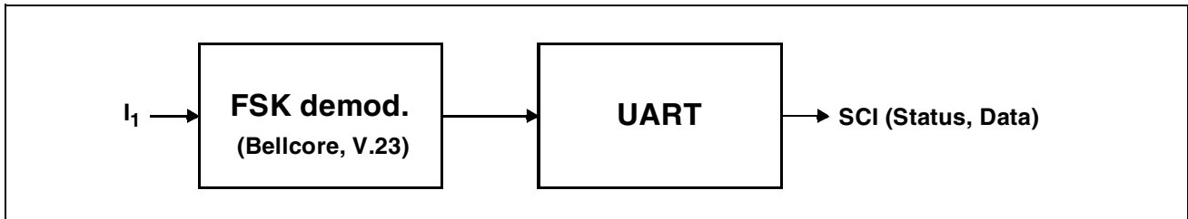
Figure 18 Caller ID Decoder - Block Diagram
