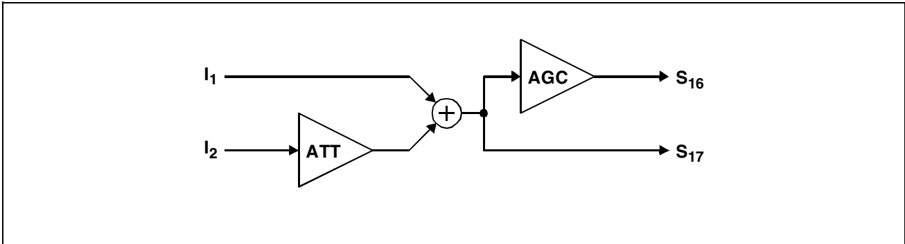
Figure 27 Automatic Gain Control Unit - Block Diagram
