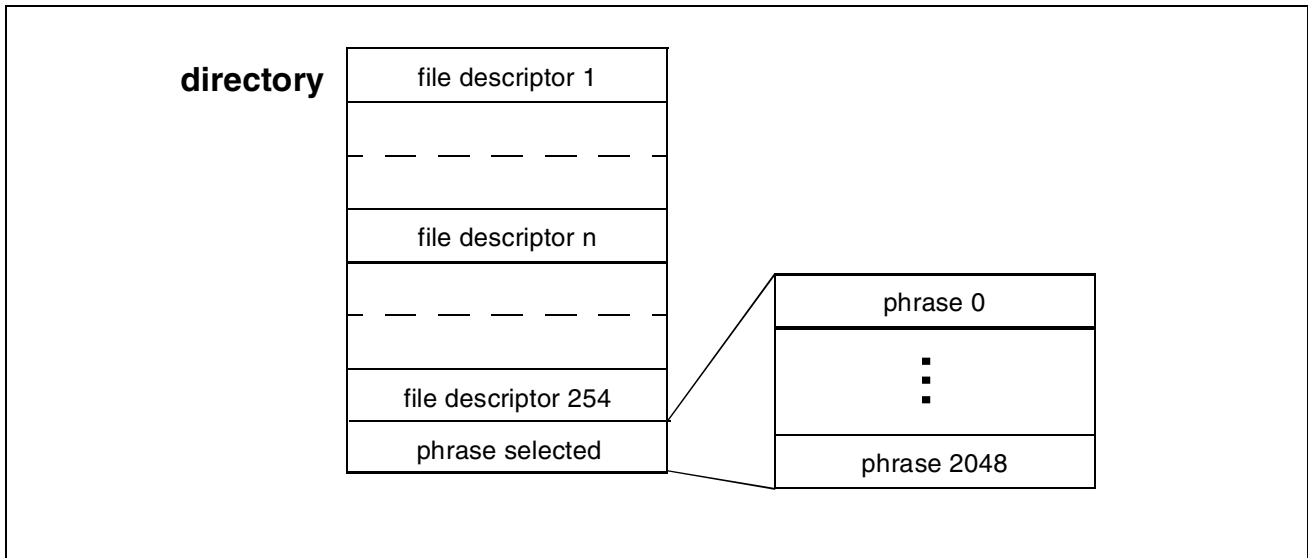
Figure 33 Memory Management - Structure of Voice Prompt Directory
