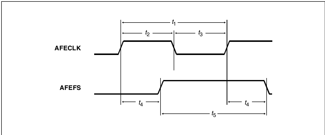
Figure 72 Clock Master Timing
