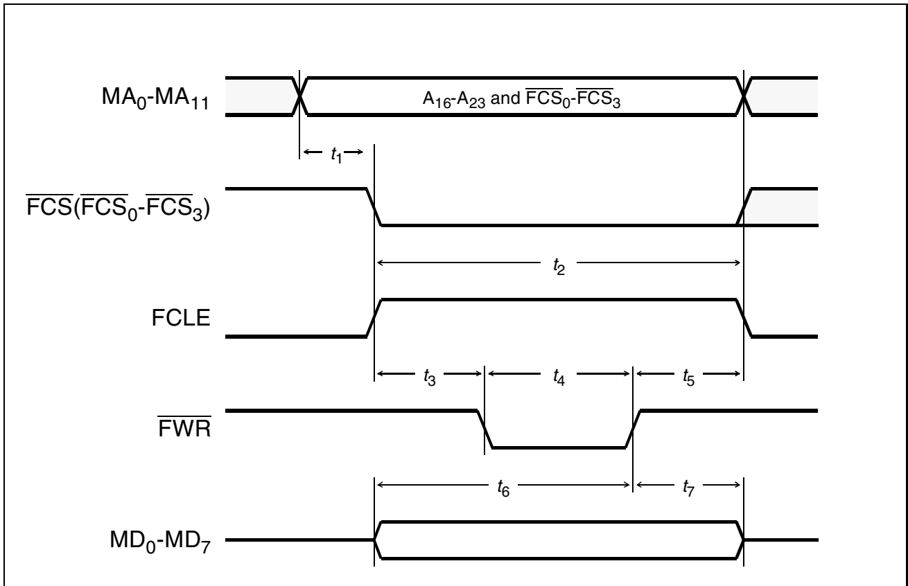
Figure 77 Memory Interface - Samsung Command Write
