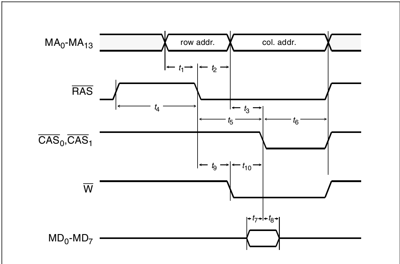
Figure 74 Memory Interface - DRAM Write Access
