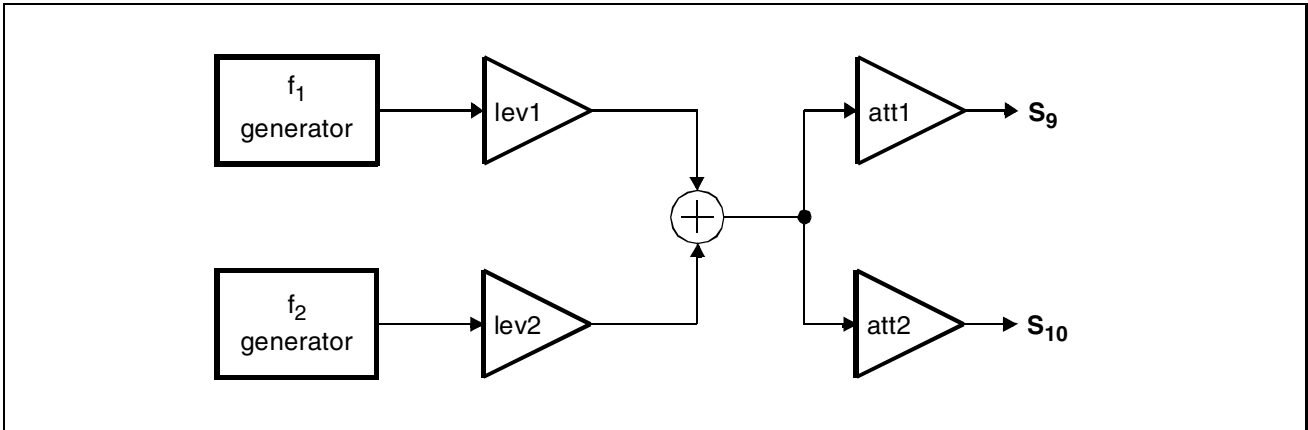
Figure 20 DTMF Generator - Block Diagram
