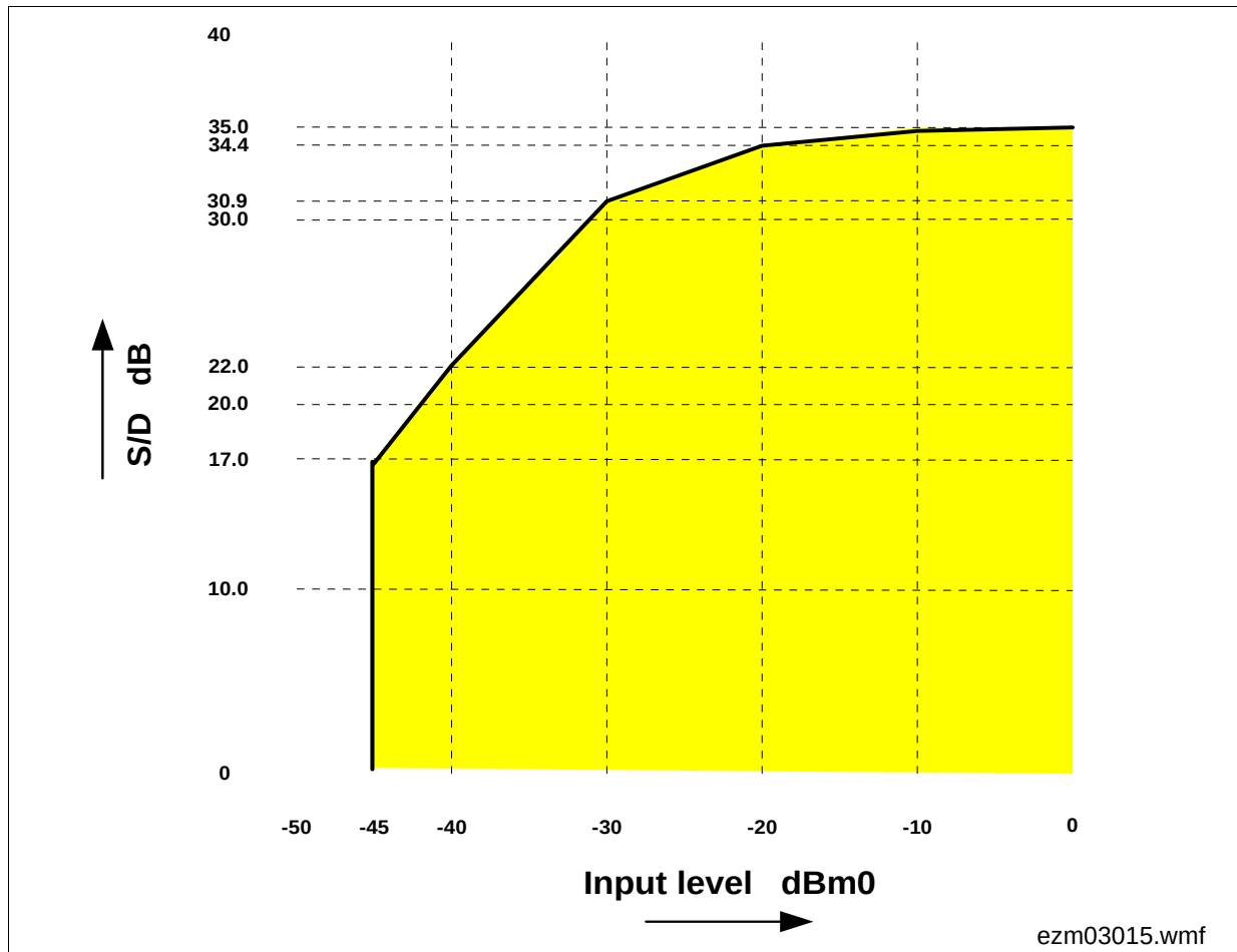
Figure 39 Total Distortion Receive AR = 7 dBr
