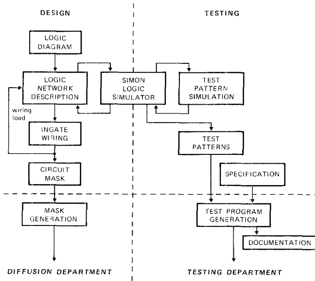
Fig. 11 CAD flow-chart.
