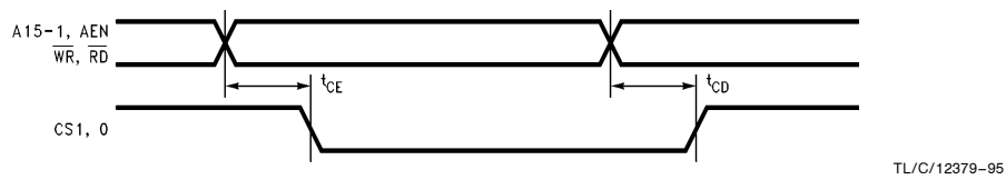
FIGURE 12-27. Chip Select Timing
