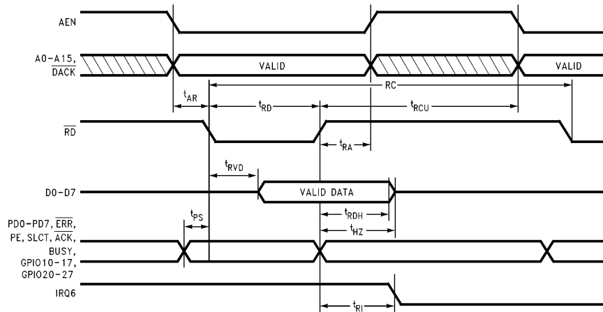
FIGURE 12-2. Microprocessor Read Timing
