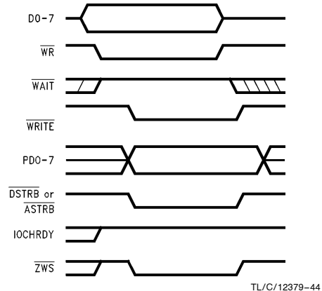
FIGURE 8-3. EPP Write with ZWS
