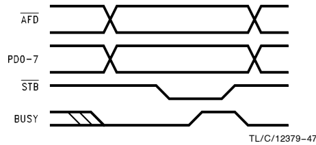
FIGURE 8-6. ECP Forward Write Cycle
