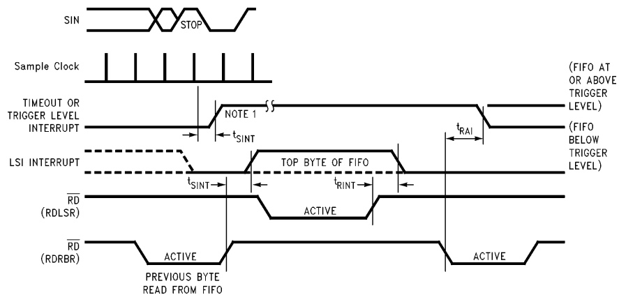
FIGURE 12-9. Timeout Receiver Timing
