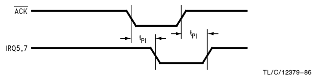
FIGURE 12-18. Compatible Mode Parallel Port Interrupt Timing
