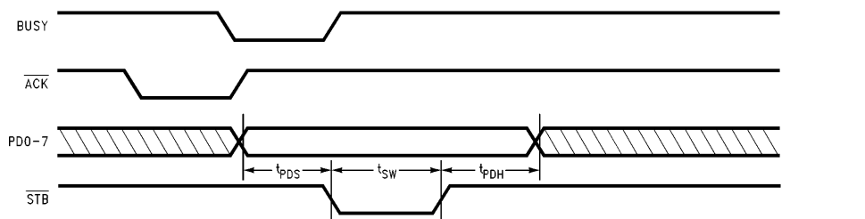
FIGURE 12-20. Typical Parallel Port Data Exchange
