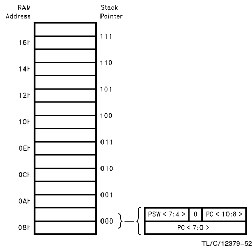
FIGURE 10-6. Keyboard Controller Stack Organization
