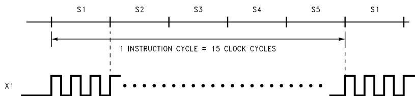
FIGURE 10-12. Instruction Cycle Timing
