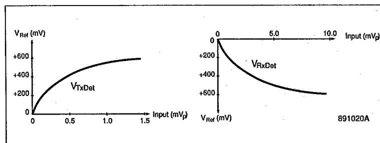
Figure 11. Transmit- and receive-channel rectifier characteristics.
