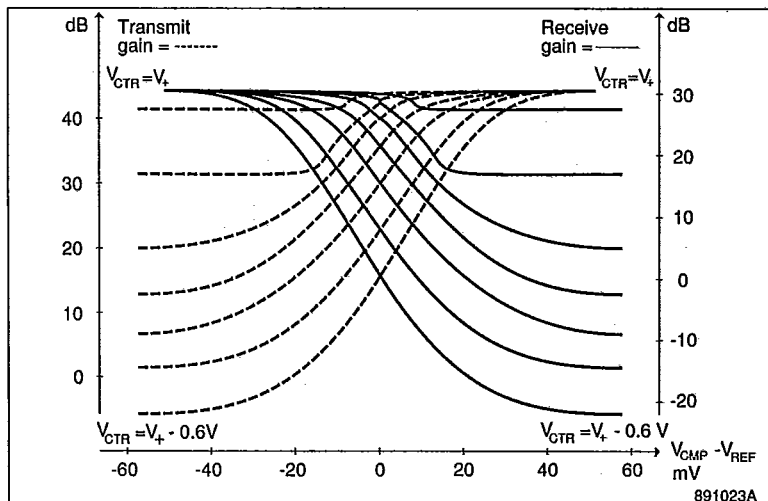
Figure 15. Transmit and receive gain as a function of V_{CMP} and V_{REF} .
