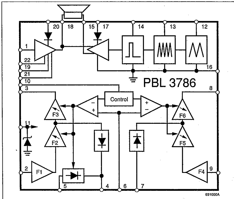
Figure 1. Block diagram.
