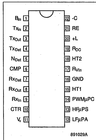
Figure 9. Pin configuration
