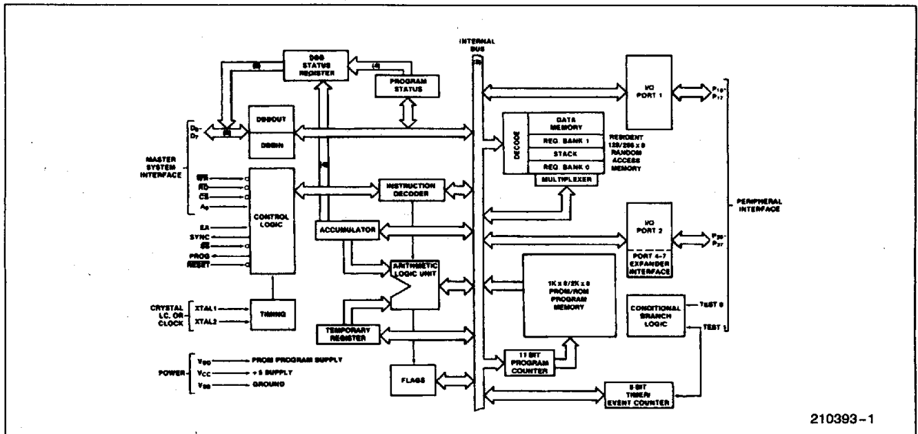
Figure 3. Block Diagram
