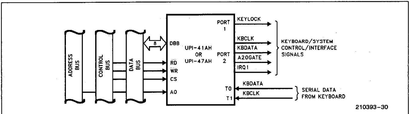
Figure 4. UPI-41AH/42AH Keyboard Controller
