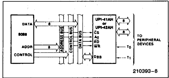
Figure 5. 8088-UPI-41AH/42AH Interface
