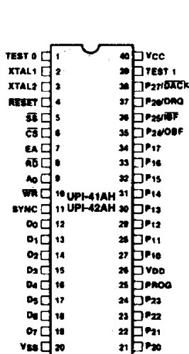
210393-2 Figure 1. DIP Pin Configuration
