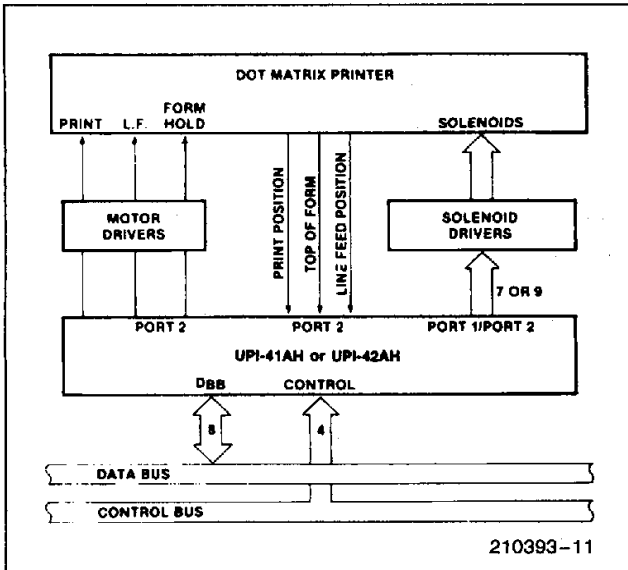
Figure 8. UPI-41AH/42AH 80-Column Matrix Printer Interface
