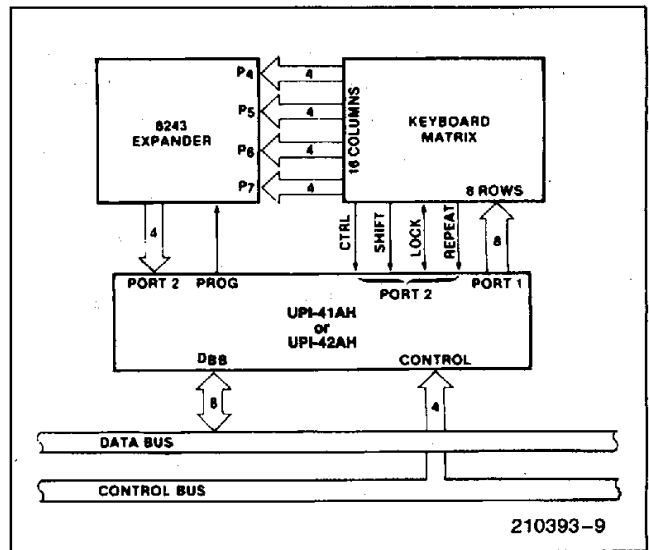
Figure 7. UPI-41/42-8243 Keyboard Scanner
