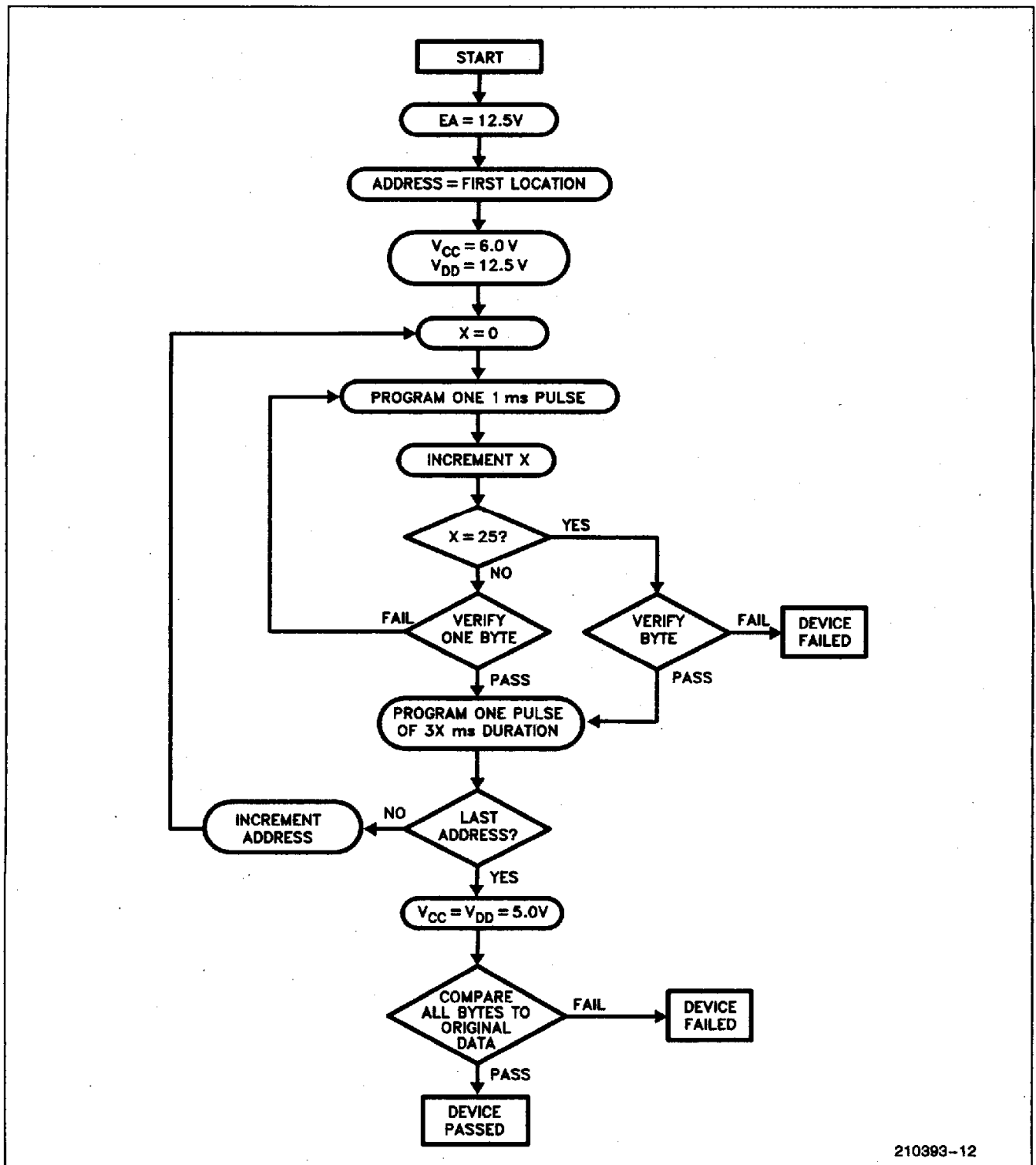
Figure 9. Programming Algorithm
