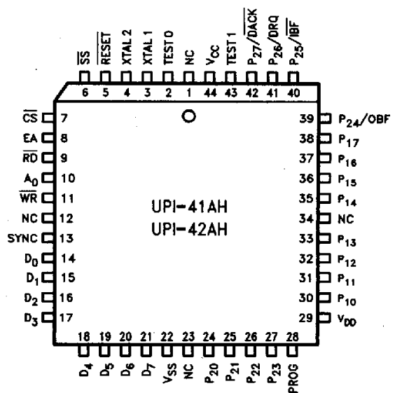
210393-3 Figure 2. PLCC Pin Configuration
