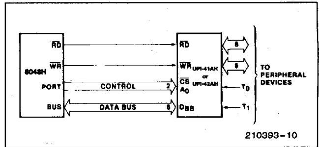
Figure 6. 8048H-UPI-41/42 Interface
