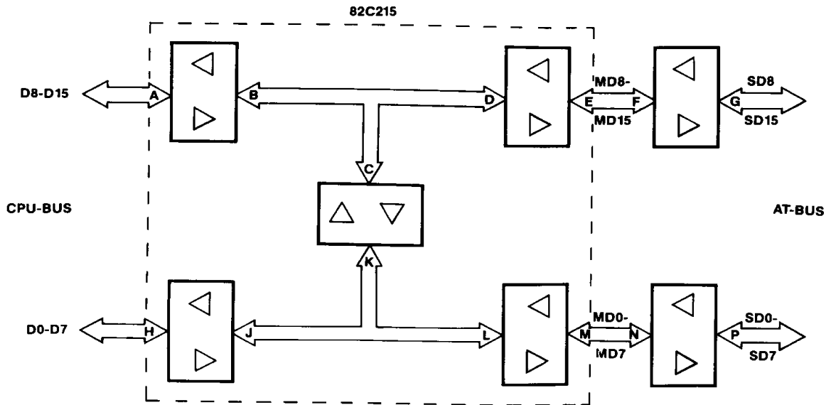
Figure 3.2 Bus Conversion Data Paths
