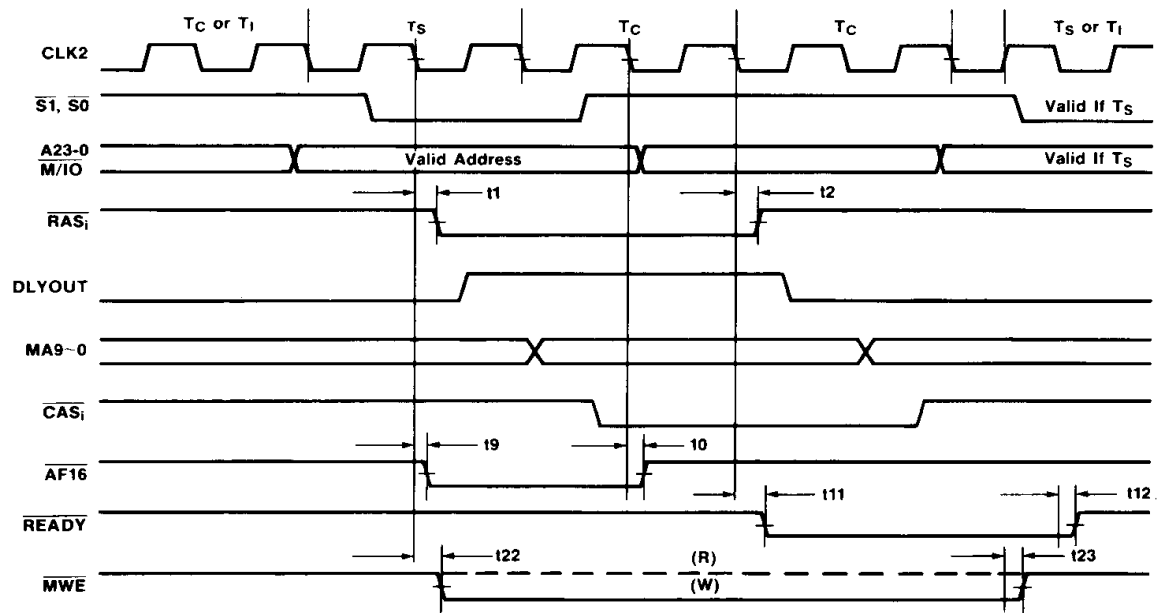
Non-Interleave Mode—1WS, Read, Write
