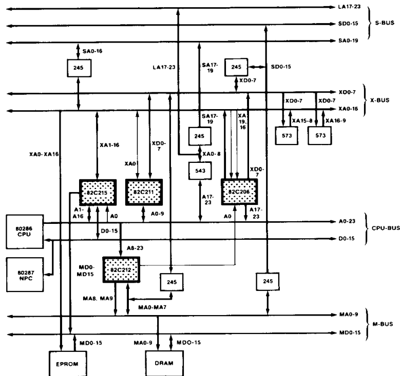
Figure 1. NEAT System Block Diagram
