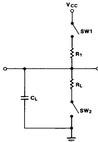
Figure 10. Load Circuit and AC Characteristics Measurement Waveform
