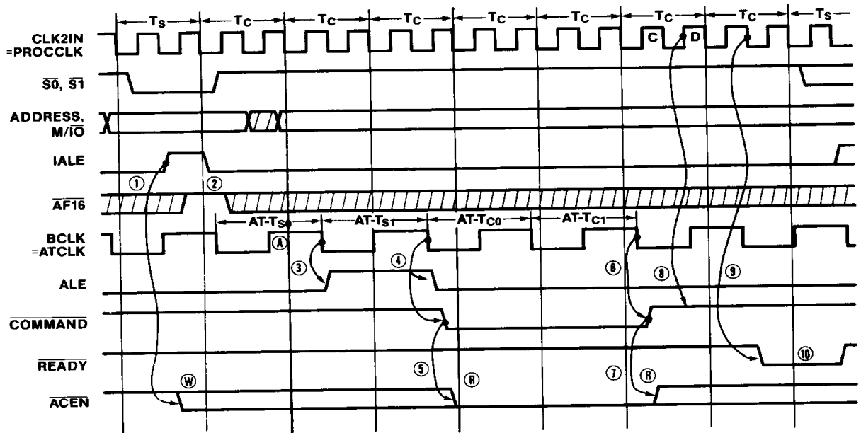
Figure 1.12 External Mode AT Bus Cycle (0WS, 0CD)
