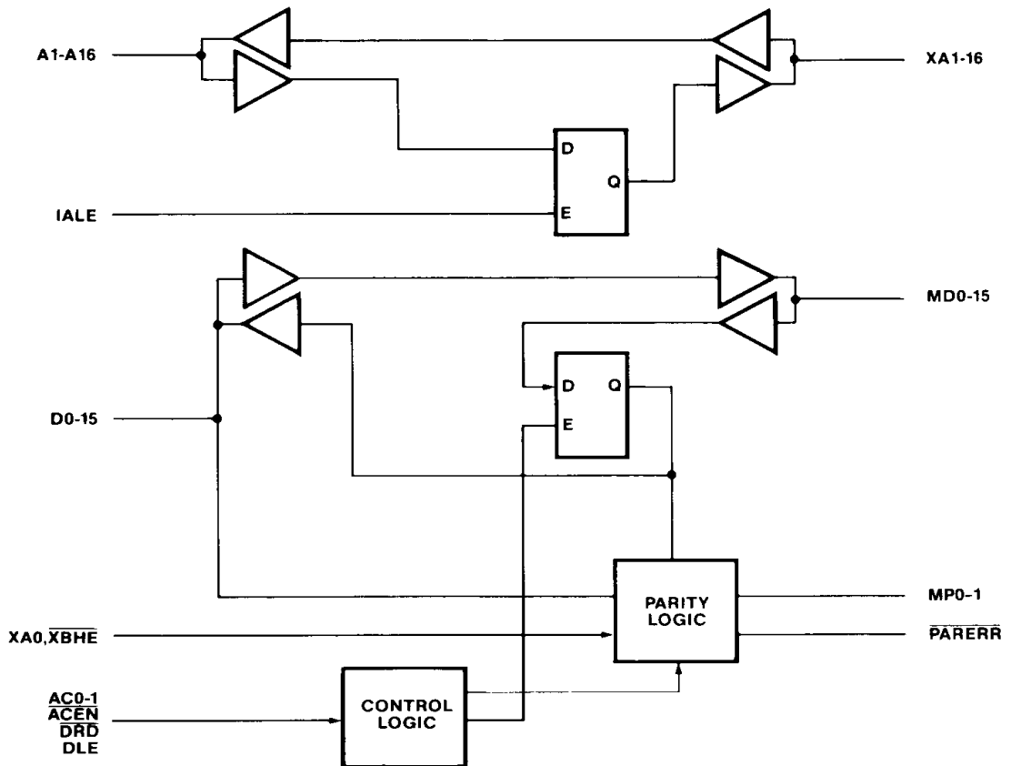
Figure 3.1 82C215 Block Diagram
