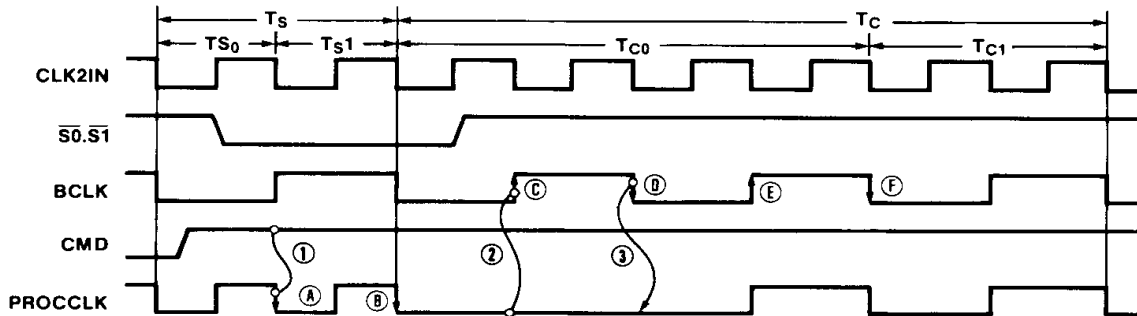
Figure 1.3 Sequence Diagram for High to Low Frequency Transition
