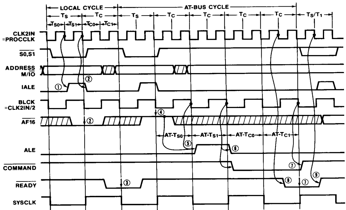
Figure 1.8 Normal Mode Local Cycle Followed by AT Bus Cycle (0WS, 0CD)
