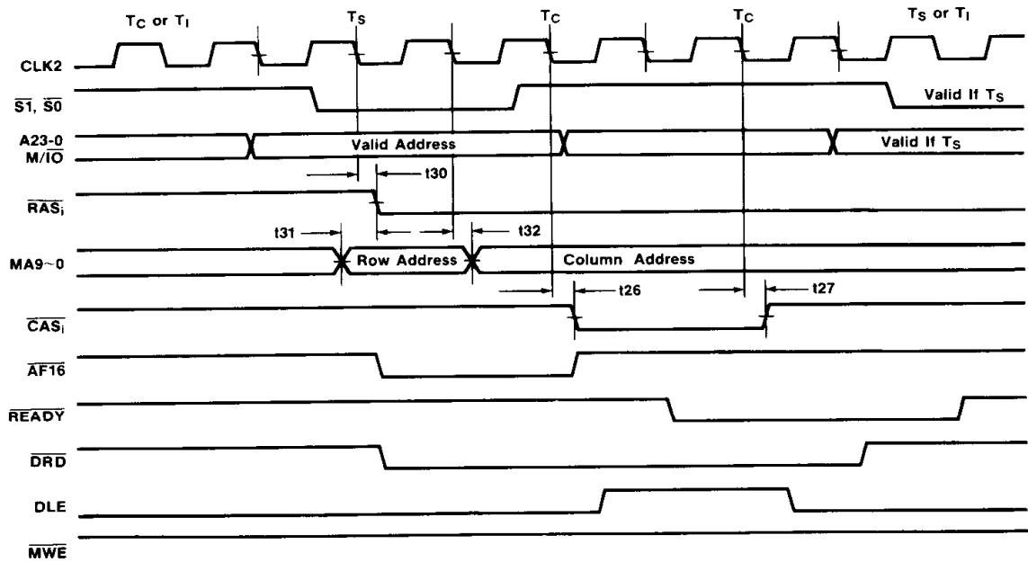
Interleave Mode—Read Cycle with RAS Being Inactive, 0WS
