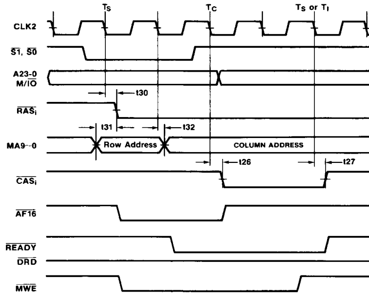
Interleave Mode—Write Cycle with RAS Being Inactive, 0WS
