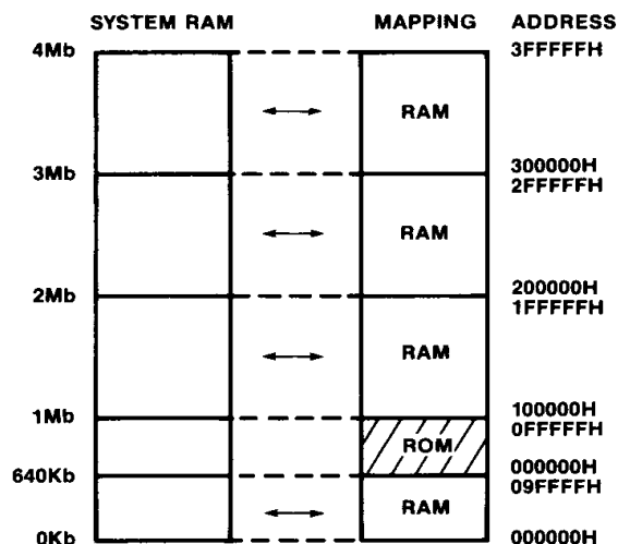
Figure 2.7 RAM/ROM Mapping Without Shadow RAM (More Than 1MB of RAM)
