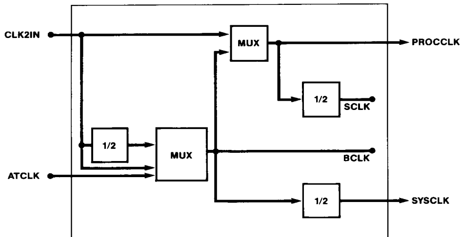
Figure 1.2 Clock Selection Block Diagram
