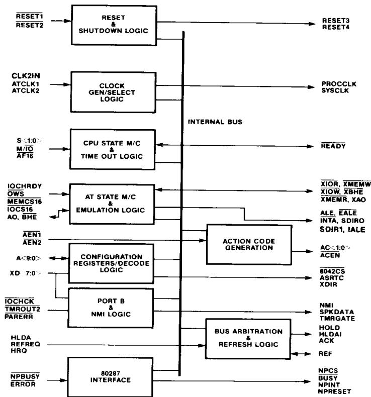
Figure 1.1 82C211 Block Diagram
