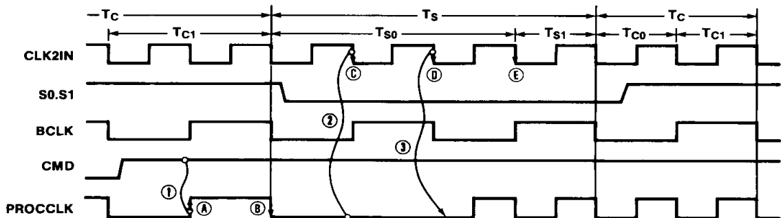
Figure 1.4 Sequence Diagram for Low to High Frequency Transition
