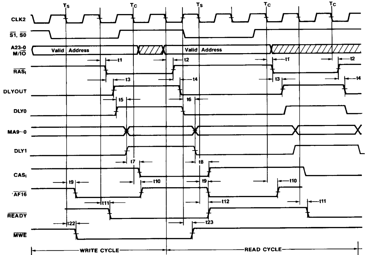
Non-Interleave Mode—Write Followed by Read, OWS
