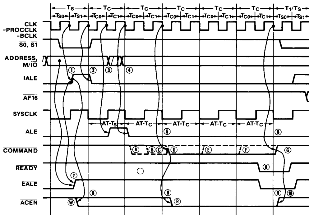
Figure 1.11 Delayed Mode AT Bus Cycle (3WS, 2CD)
