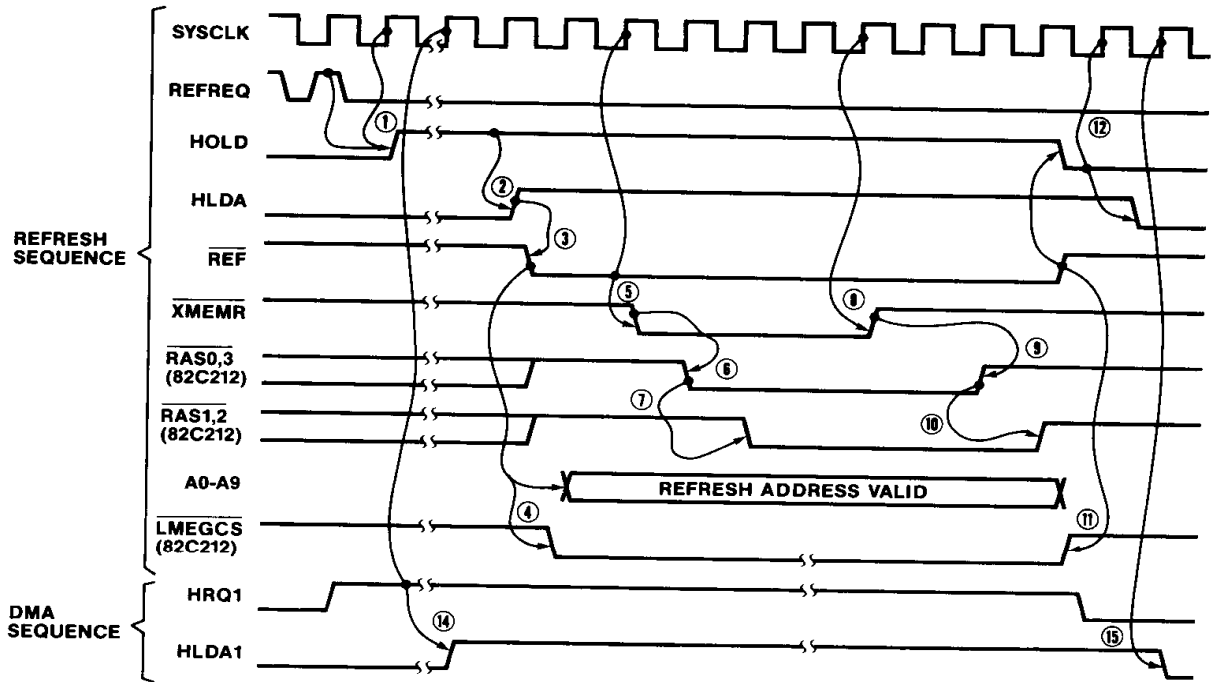
Figure 1.5 Refresh/DMA Sequence
