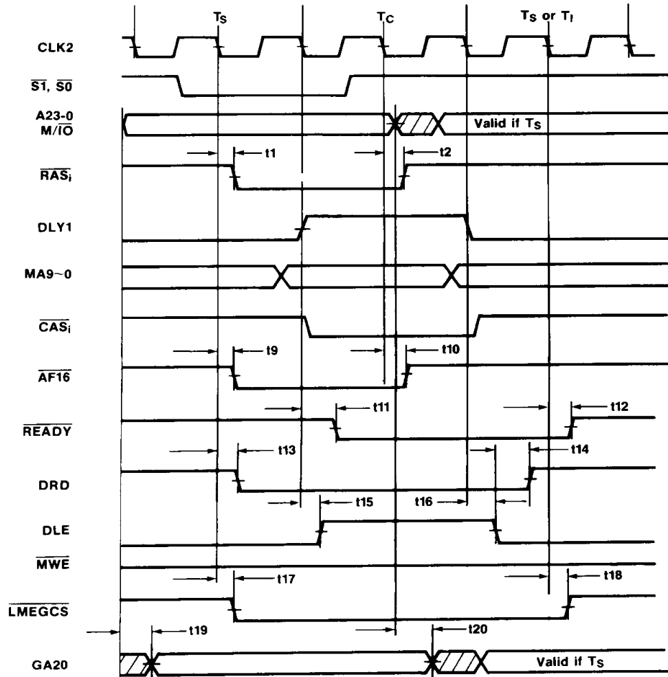
Non-Interleave Mode—Read, 0WS
