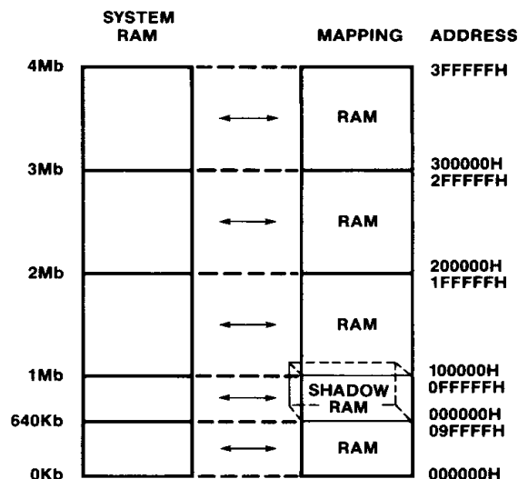
Figure 2.8 RAM Mapping with Shadow RAM (More Than 1MB of RAM)
