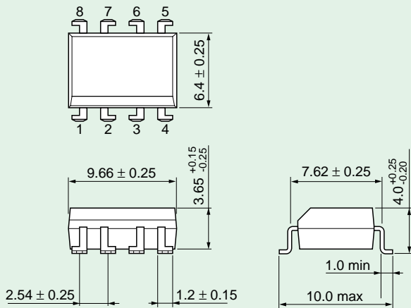
DIP8 (LF4)
