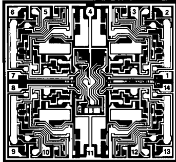
DIE SIZE 0.093 × 0.087 inch, 8091 sq. mils (2.36 × 2.21 mm, 5.22 sq. mm)
