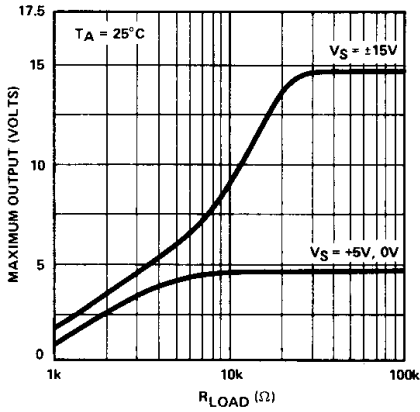
MAXIMUM OUTPUT VOLTAGE vs LOAD RESISTANCE
