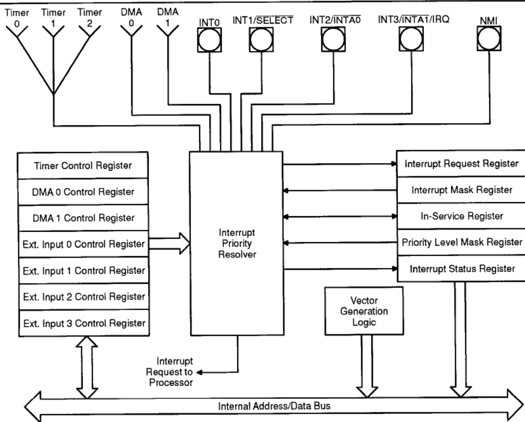
Figure 19. Interrupt Controller Block Diagram
