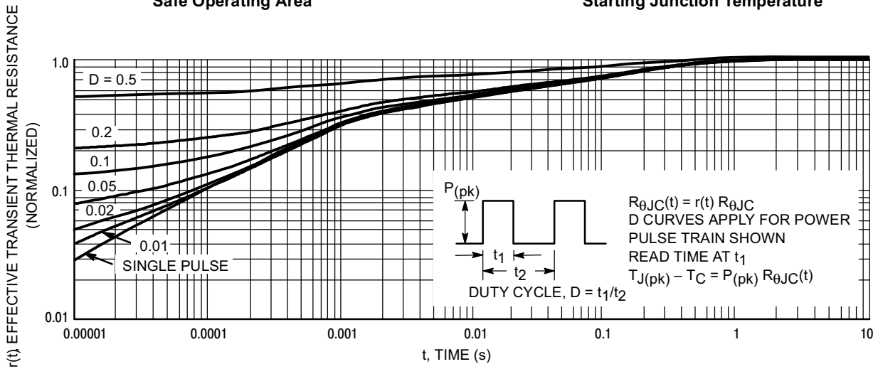
Figure 13. Thermal Response
