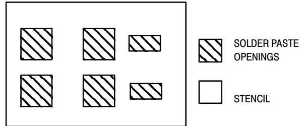
Figure 15. Typical Stencil for DPAK and D 2 PAK Packages
