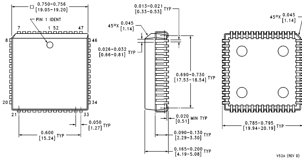
52-Lead Molded Plastic Leaded Chip Carrier Package Number V52A Order Number NM95MS16V
