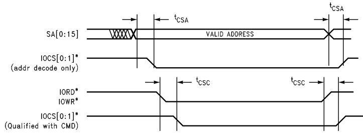
Decode Delay for Chipselect Generation
