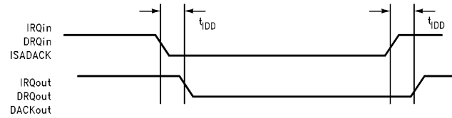
Propagation Delay for IRQ/DRQ/DACK
