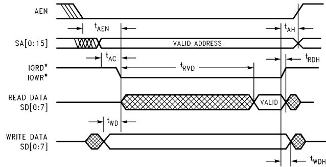
Timings for ISA Read/Write Cycle
