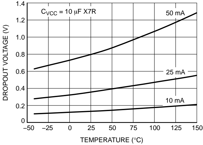
Figure 19. Dropout Voltage vs. Temperature
