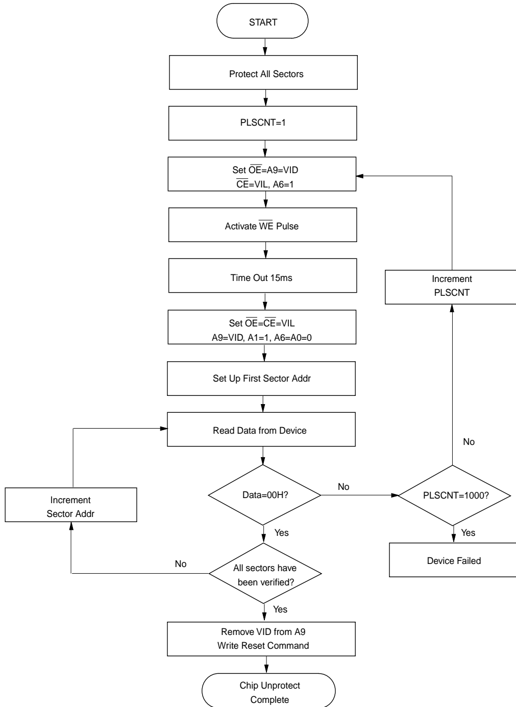
Fig 17. CHIP UNPROTECT FLOWCHART(A9, \overline{OE} Control)
