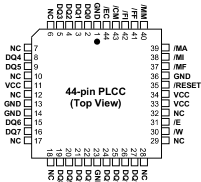
Figure 1: Pinout Diagram
