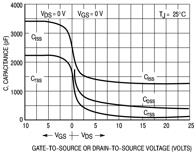
Figure 7. Capacitance Variation
