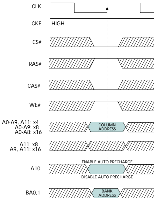
Figure 5 READ Command
