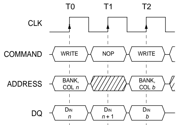
Figure 14 WRITE BURST
