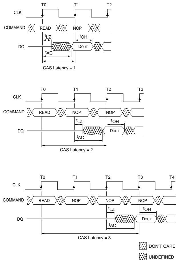
Figure 6 CAS LATENCY
