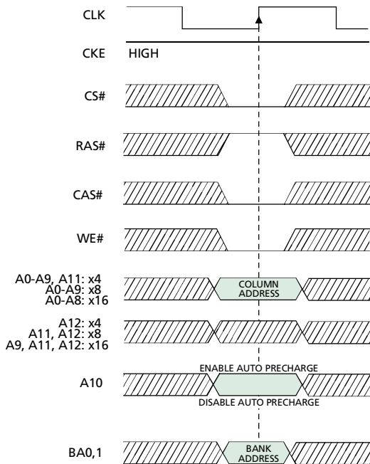
Figure 13 WRITE Command
