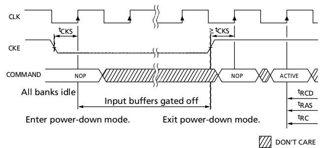
Figure 21 Power-Down
