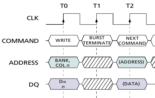
Figure 19 Terminating a WRITE Burst
