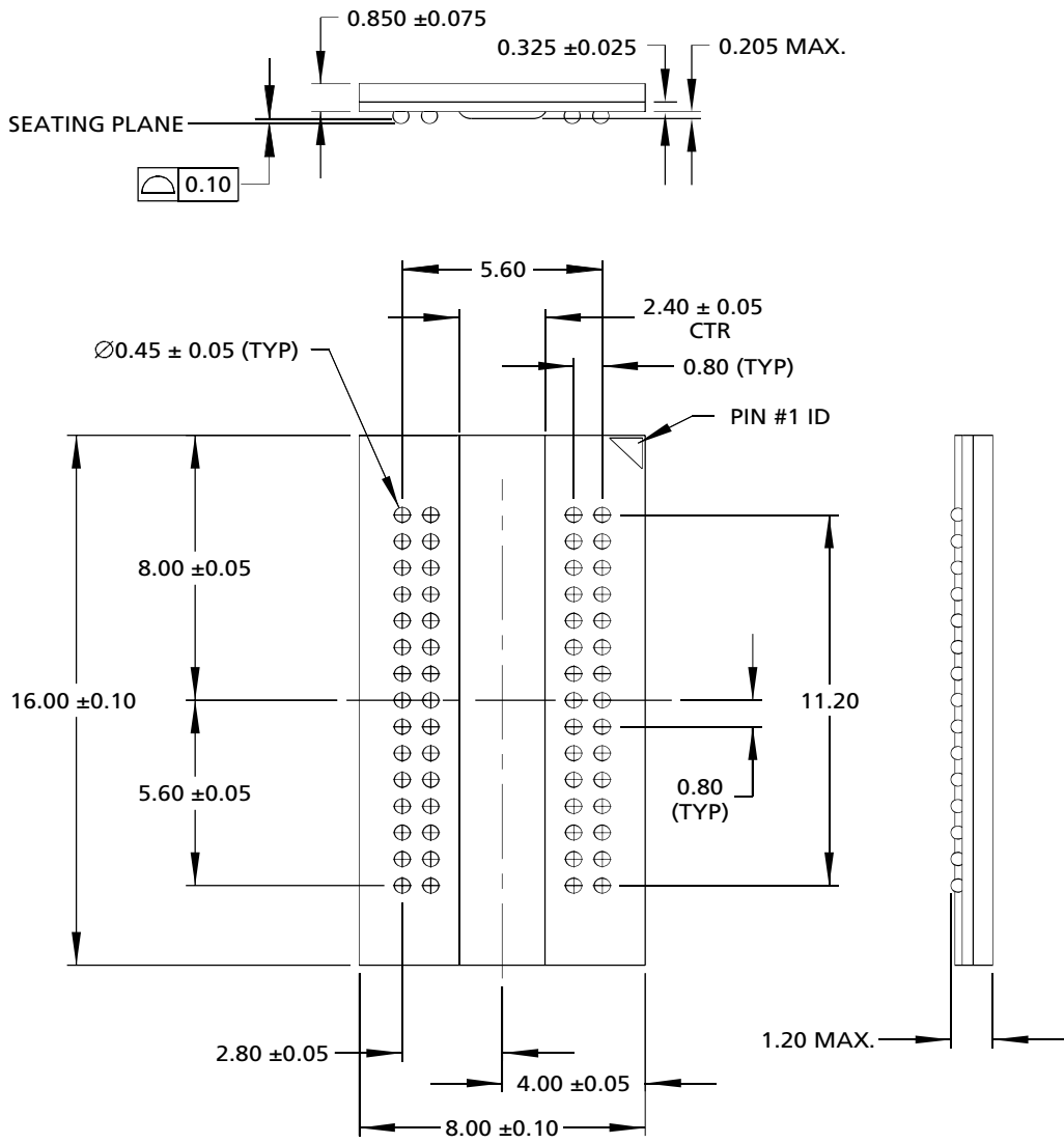
(Bottom View)
