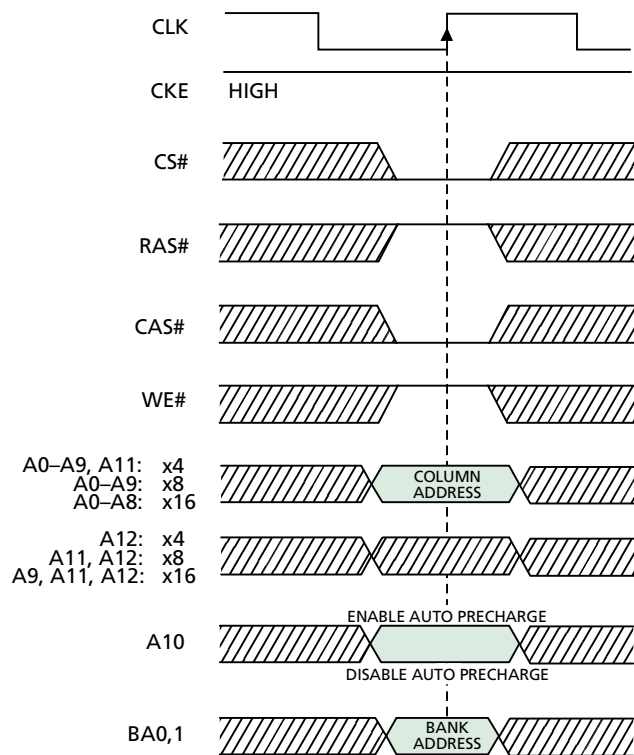
Figure 5 READ Command
