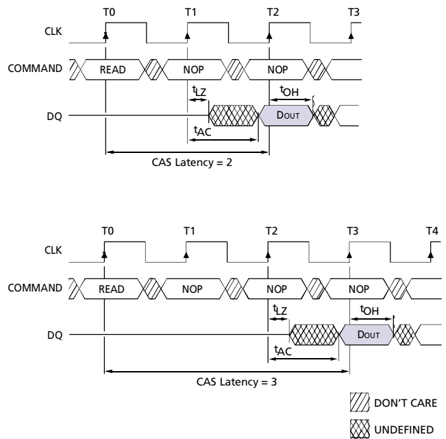
Figure 6 CAS Latency
