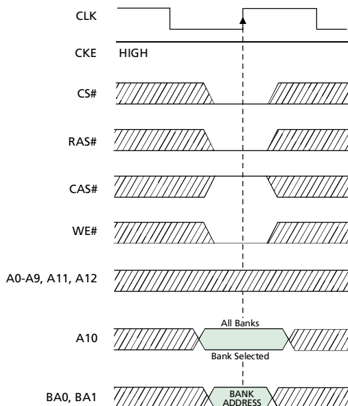
Figure 20 PRECHARGE Command
