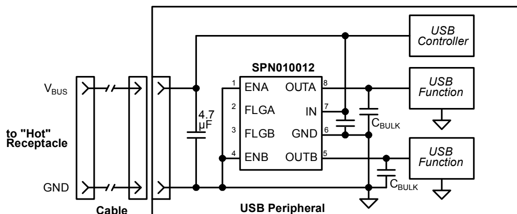
Figure 3. Hot-Plug Application
