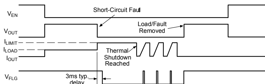
Figure 2. MIC2026-2 Fault Timing
