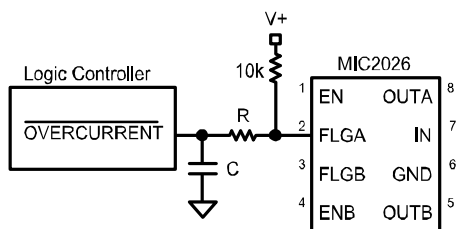
Figure 4. Transient Filter
