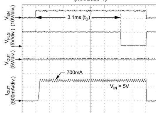
Enabled Into Short (MIC2026-1)
