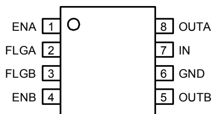
8-Pin SOIC (M) 8-Pin DIP (N)
