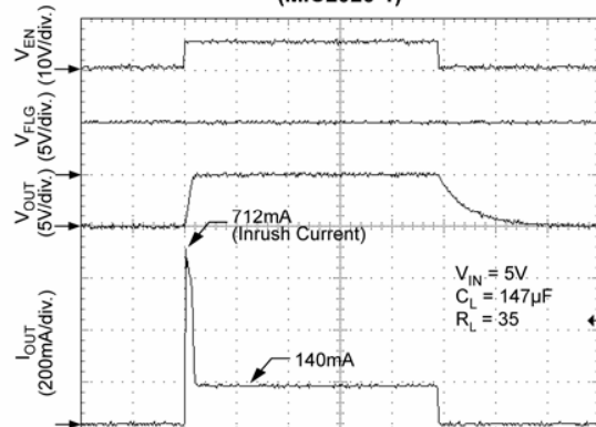
Turn-On/Turn-Off (MIC2026-1)
