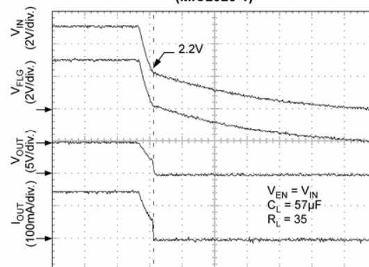
UVLO— V_{IN} Falling (MIC2026-1)
