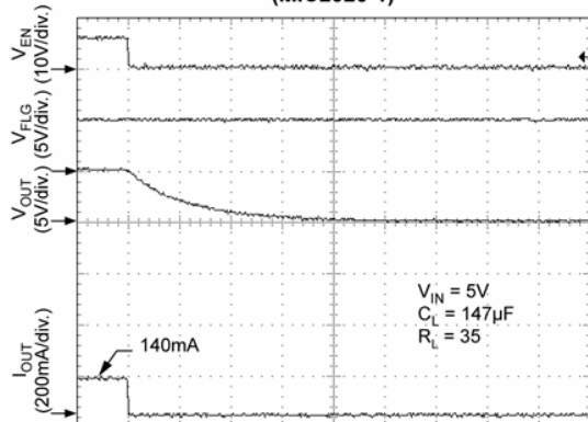
Turn-Off (MIC2026-1)
