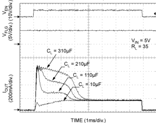
Inrush Current Response (MIC2025-1)
