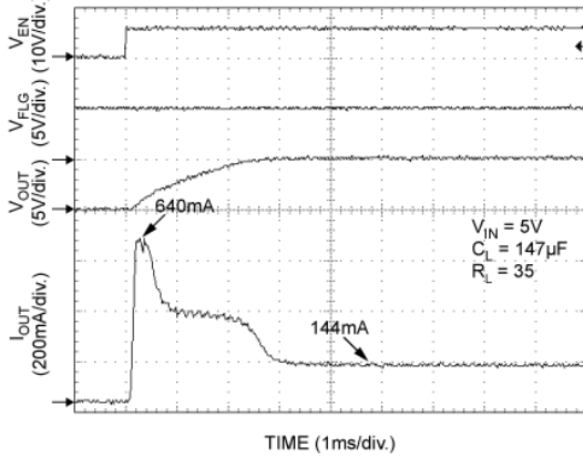
Turn-On Response (MIC2025-1)
