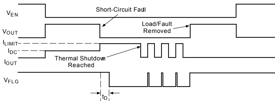
Figure 2. MIC2025-2 Timing
