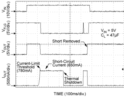
Current-Limit Response (Ramped Load Into Short—MIC2025-1)
