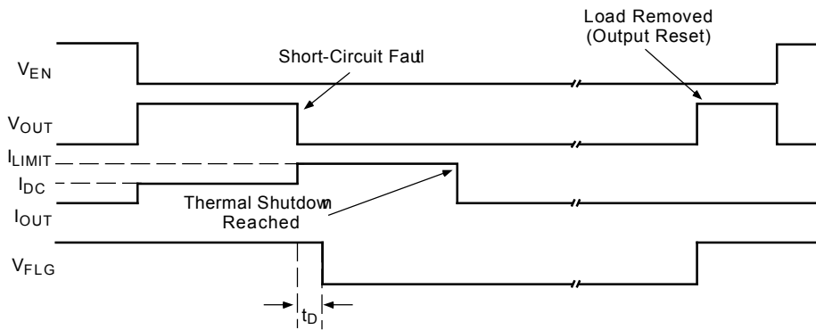
Figure 1. MIC2075-2 Timing: Output Reset by Removing Load
