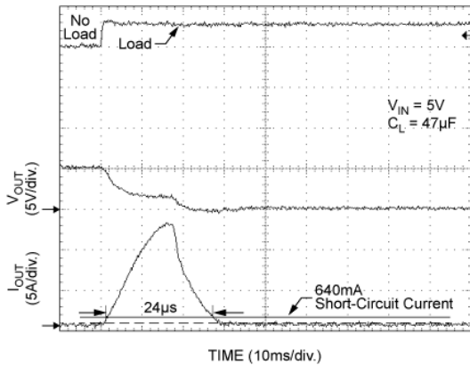
Current-Limit Transient Response (MIC2025-1)
