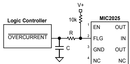
Figure 4. Transient Filter
