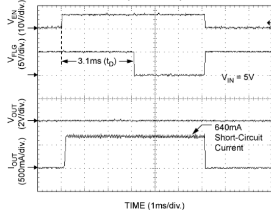
Enable Into Short (MIC2025-1)
