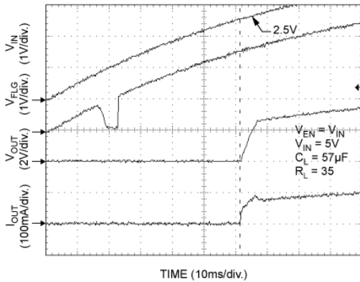
UVLO— V_{IN} Rising (MIC2025-1)
