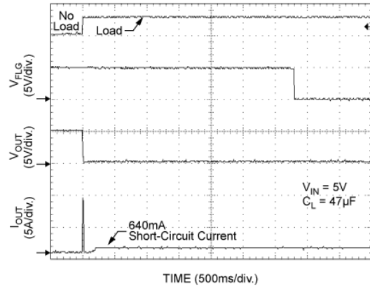
Current-Limit Transient Response (Enable Into Short—MIC2025-1)
