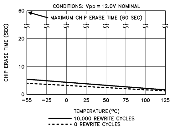
Figure 9. M28F010 Typical Erase Time vs. Temperature
