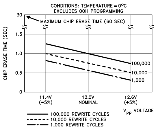
Figure 10. M28F010 Typical Erase Time vs. V_{pp} Voltage
