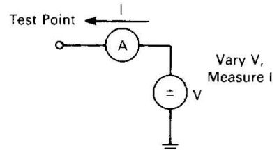
Figure 18. I/O Characteristic Measurement Circuit
