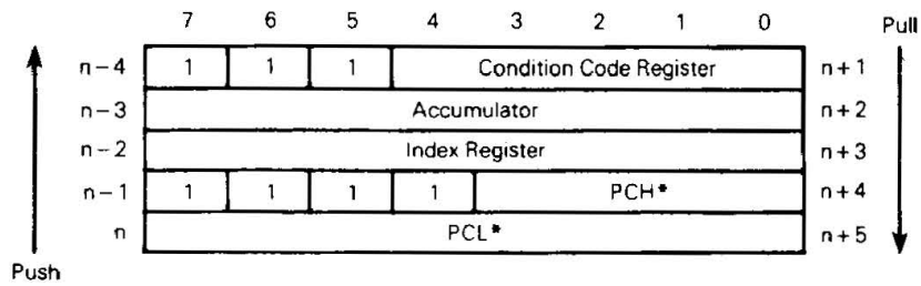
Figure 6. Interrupt Stacking Order
