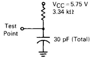
Figure 14. Open-Drain Equivalent Test Load (Port C)
