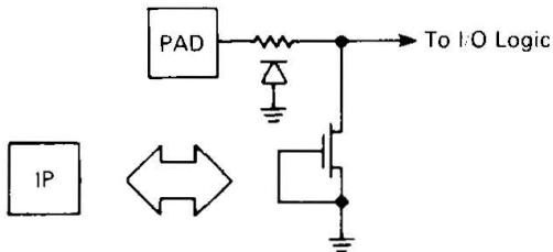
Port 17. Typical Input Protection
