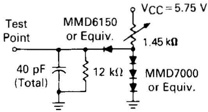
Figure 11. TTL Equivalent Test Load (Port B)
