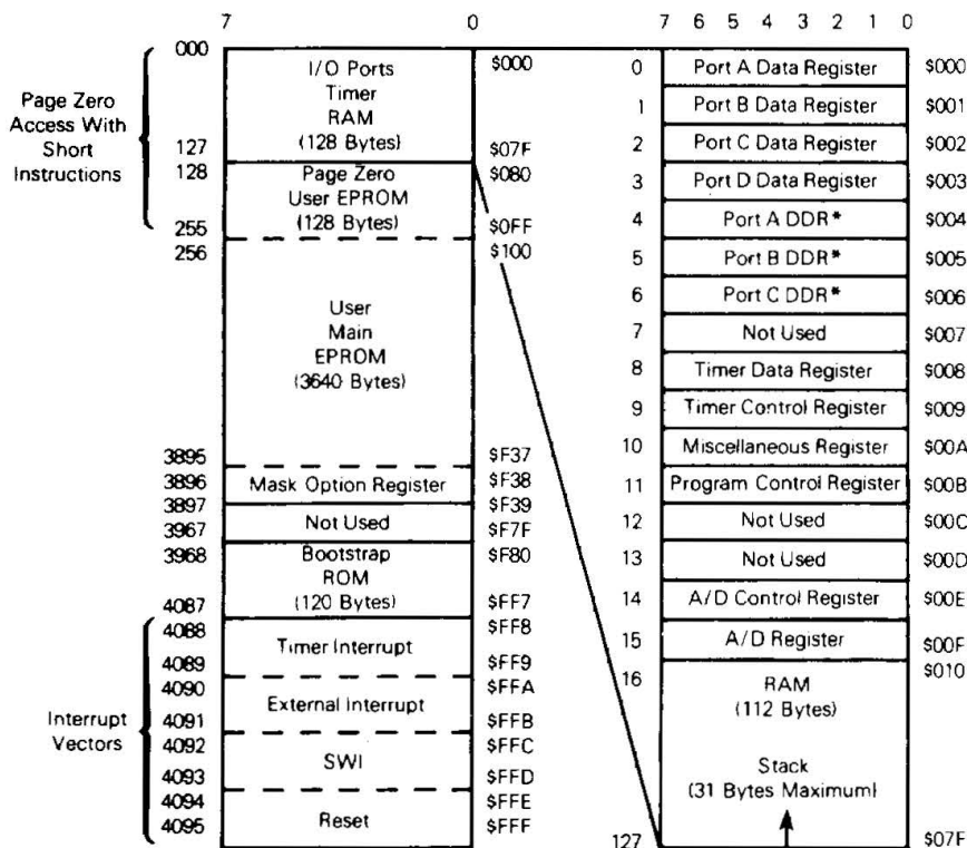
Figure 4. Memory Map
