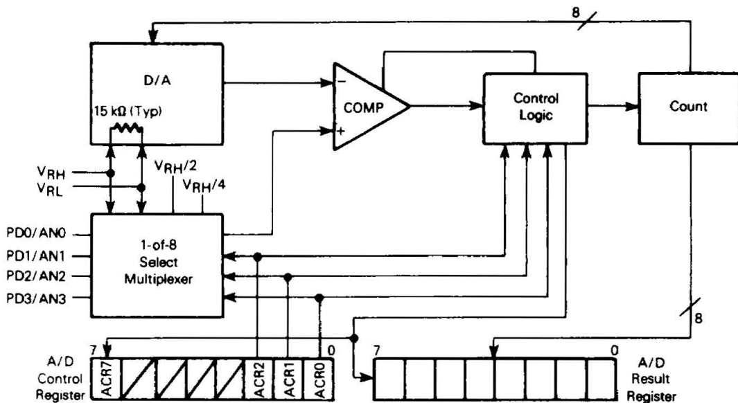
Figure 10. A/D Block Diagram
