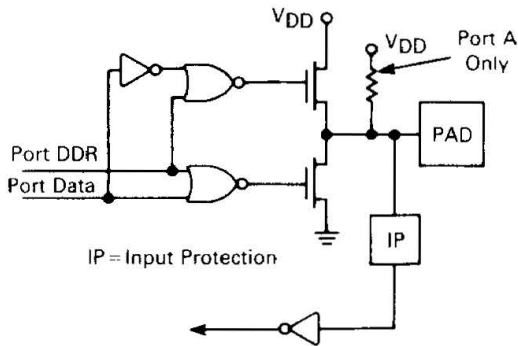
Figure 15. Ports A and C Logic Diagram
