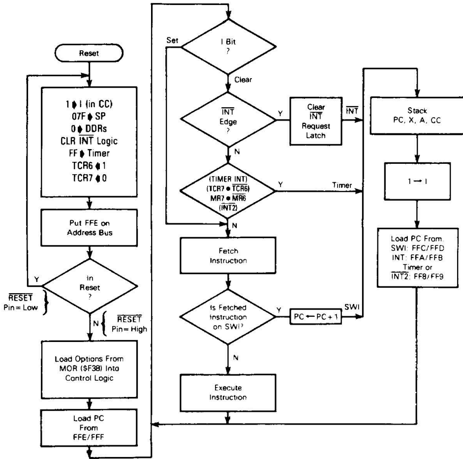
Figure 7. Reset and Interrupt Processing Flowchart
