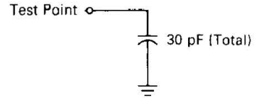
Figure 12. CMOS Equivalent Test Load (Port A)
