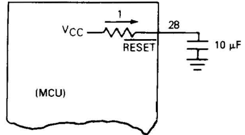
Figure 5. Power-Up \overline{\text{RESET}} Delay Circuit
