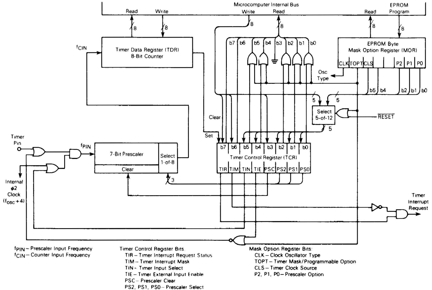
Figure 9. Timer Block Diagram
