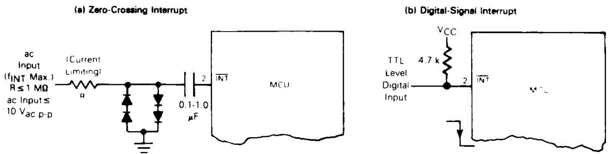
Figure 8. Typical Interrupt Circuits
