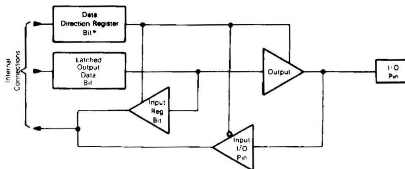
Figure 3. Typical Port I/O Circuitry and Register Configuration
