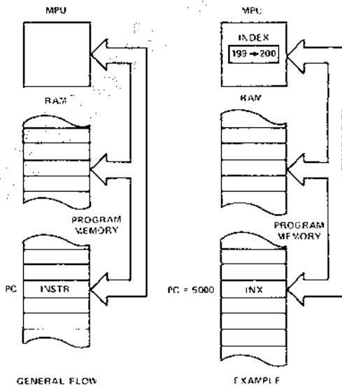
FIGURE 27 -- INHERENT ADDRESSING
