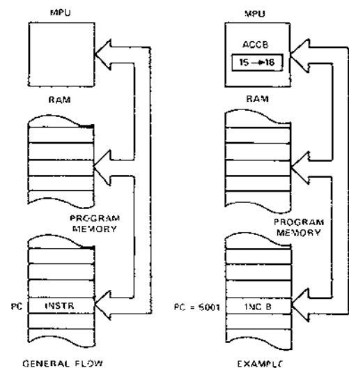
FIGURE 28 -- ACCUMULATOR ADDRESSING
