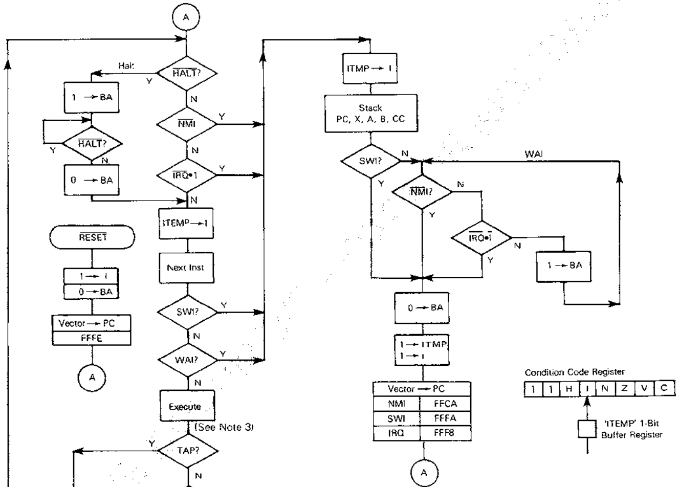
FIGURE 10 - MPU FLOWCHART
