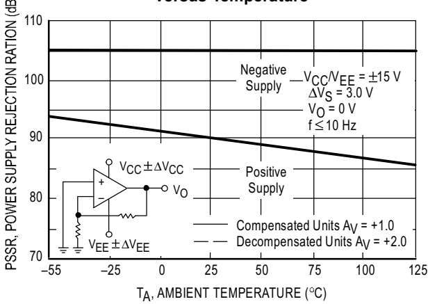
Figure 30. Power Supply Rejection Ratio versus Temperature
