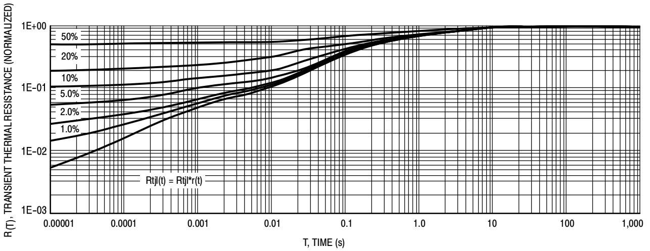
Figure 9. Thermal Response Junction to Lead
