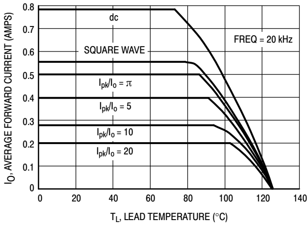
Figure 5. Current Derating
