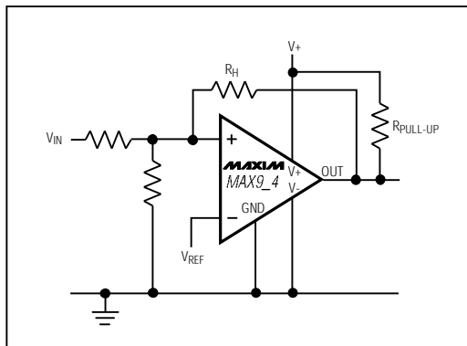
Figure 4. External Hysteresis
