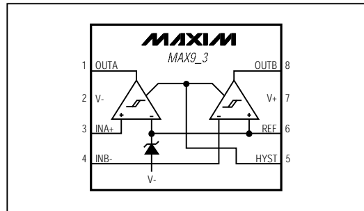
Figure 1c. MAX973/MAX983 Functional Diagram (Window Comparator)
