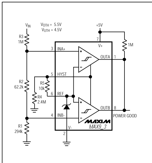
Figure 5. Window Detector
