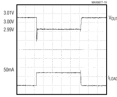
MAX8877-19 10µs/div MAX887_EUK30, V_{IN} = V_{OUT} + 0.5V , C_{IN} = 10\mu F , I_{LOAD} = 0mA TO 50mA
