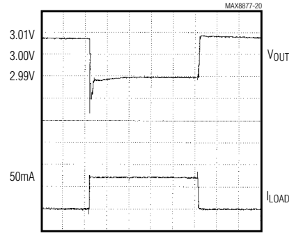
MAX8877-20 10µs/div MAX887_EUK30, V_{IN} = V_{OUT} + 0.1V , C_{IN} = 10\mu F , I_{LOAD} = 0mA TO 50mA
