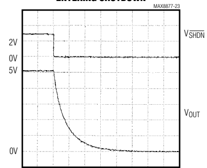
MAX8877-23 500µs/div MAX8878, NO LOAD
