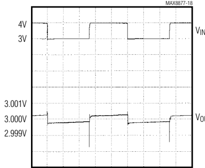
MAX8877-18 100µs/div MAX887_EUK30, I_{LOAD} = 50mA
