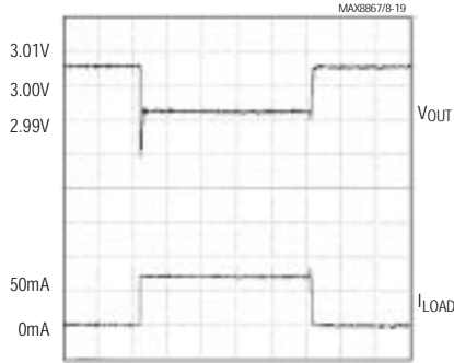
10 \mu s /div MAX886_EUK30, V_{IN} = V_{OUT} + 0.5V , C_{IN} = 10\mu F , I_{LOAD} = 0mA TO 50mA
