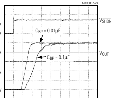
5 \mu s /div I_{LOAD} = 50mA
