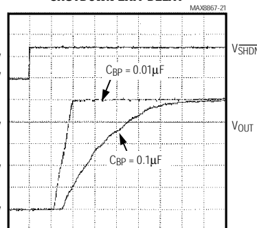
5 \mu s /div I_{LOAD} = 50mA
