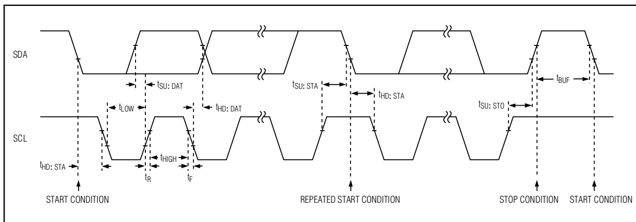
Figure 3. 2-Wire Serial Interface Timing Diagram
