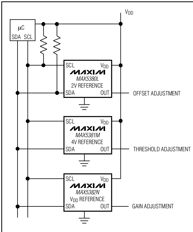
Figure 7. Typical I 2 C Application
