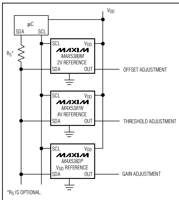
Figure 4. Typical Application Circuit
