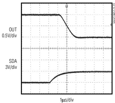
MAX5380
