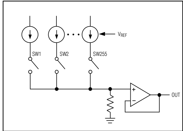
Figure 2. Current-Steering Topology
