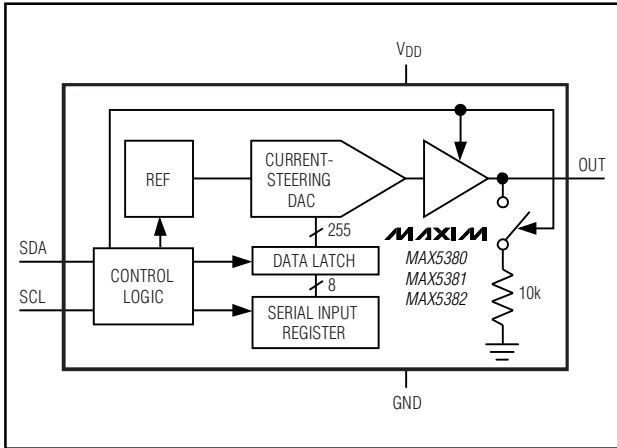
Figure 1. Functional Diagram
