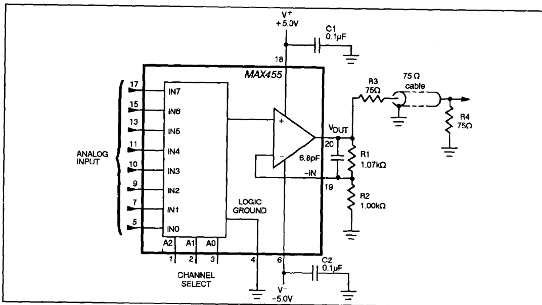
Figure 1. Typical Application
