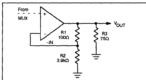
Figure 2. Unity-Gain Connections
