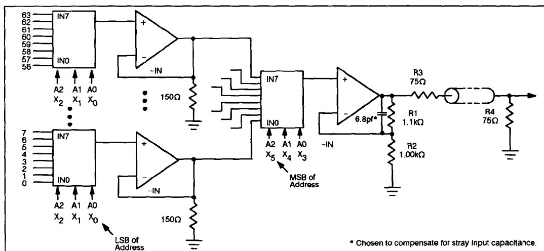
Figure 3. Nine MAX455s Used to Multiplex 64 Channels.
