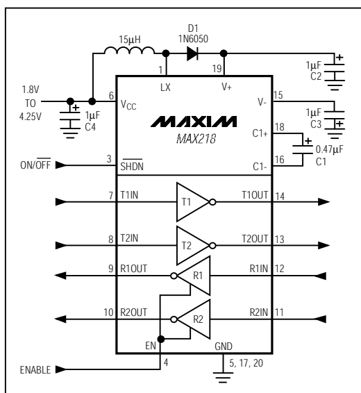
Figure 1. Single-Supply Operation
