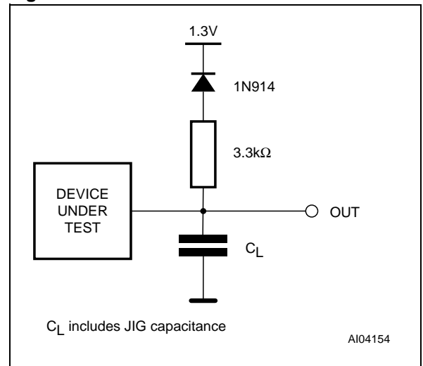
Figure 8. AC Measurement Load Circuit
