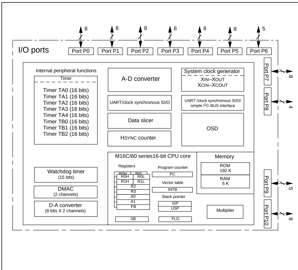
Figure 1.4.1 Block diagram
