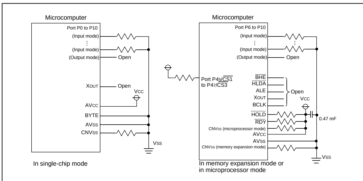
Figure 2.17.18 Example connection of unused pins
