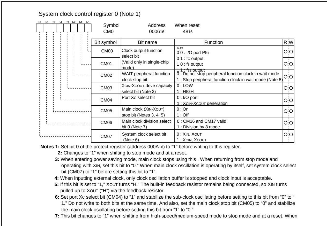
Figures 2.5.5 System clock control register 0
