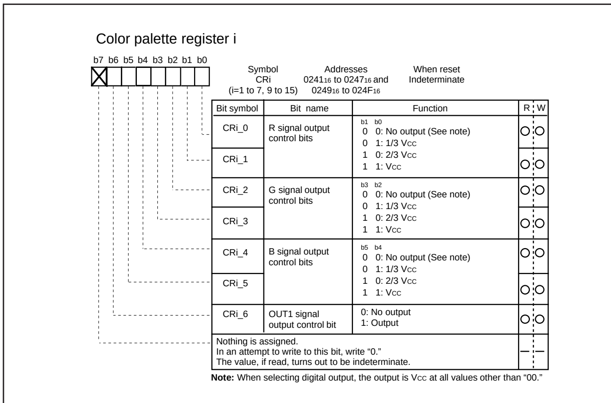
Figure 2.16.30 Color palette register i (i = 1 to 7, 9 to 15)
