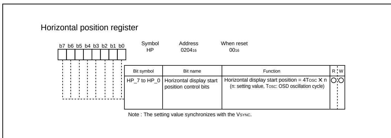
Figure 2.16.11 Horizontal position register
