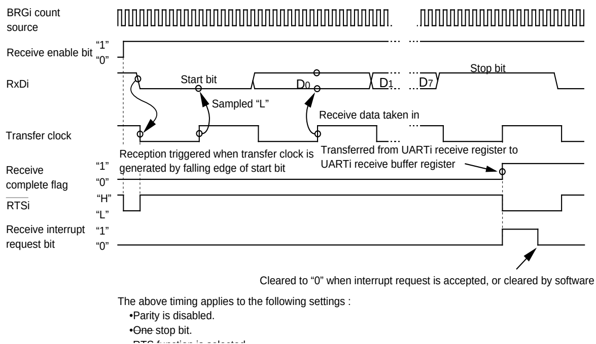
Figure 2.11.23 Typical transmit/receive timings in UART mode
