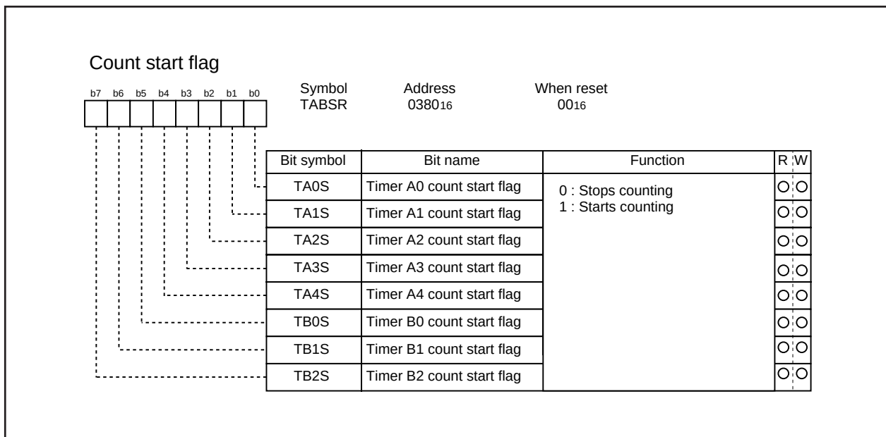
Figure 2.10.6 Count start flag
