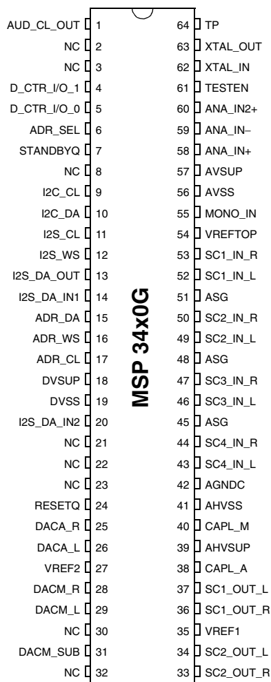
Fig. 4–6: PSDIP64-1 package
