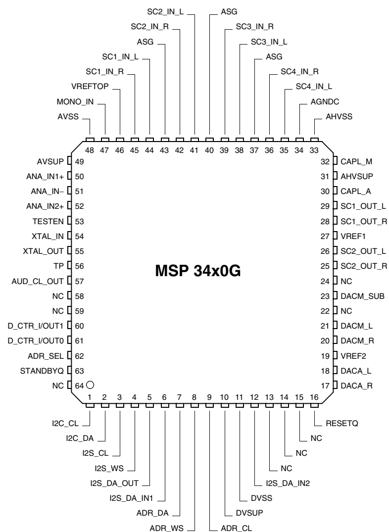
Fig. 4-9: PMQFP64-2 package
